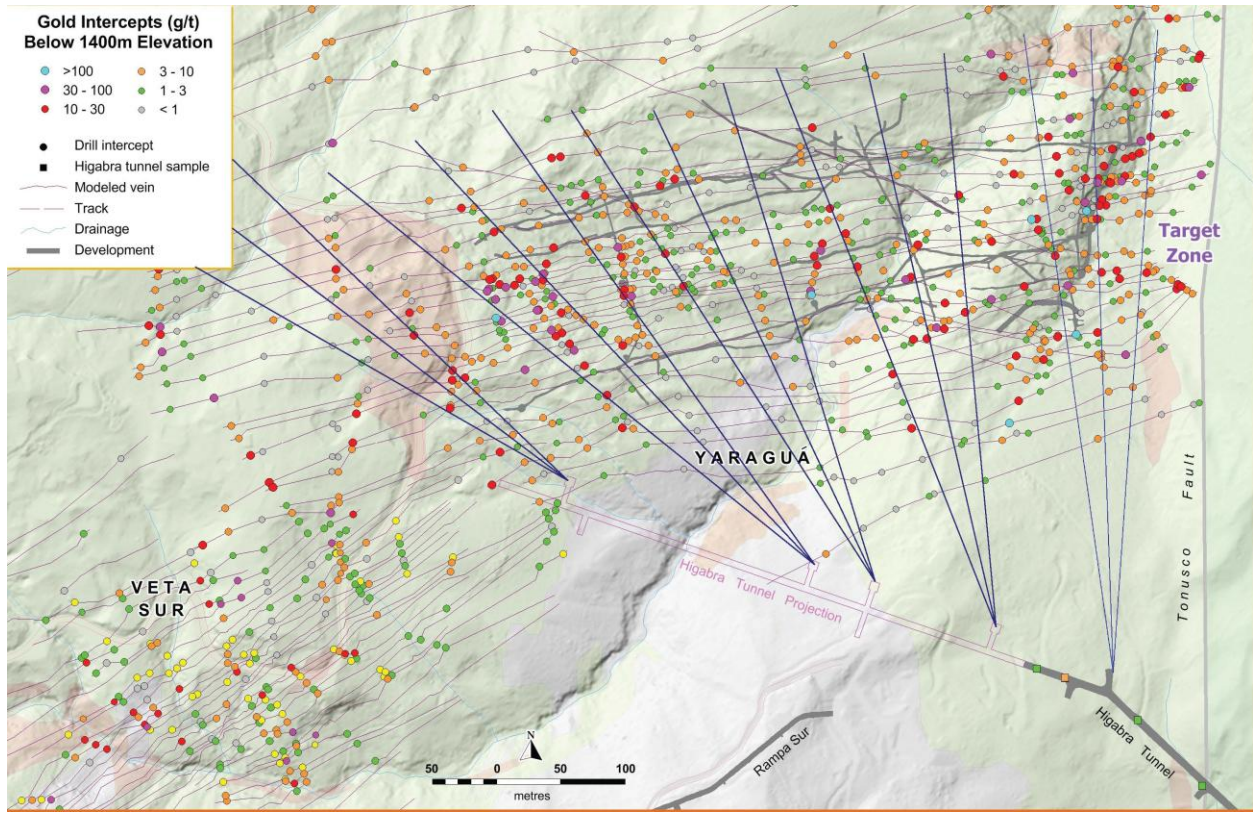
Figure 1: Higabra Valley Tunnel Exploration Drilling Program FY2014
