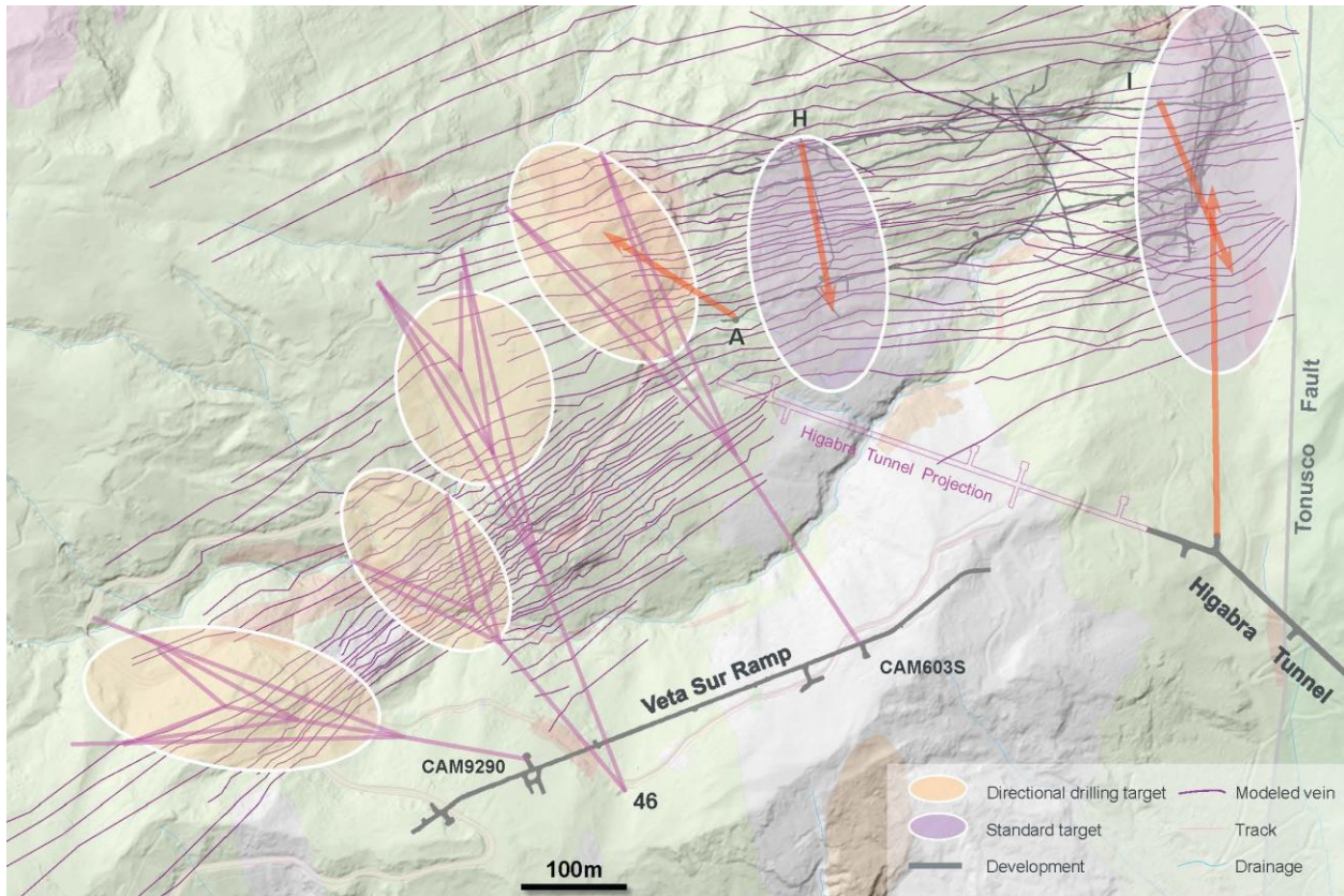
Figure 2: Veta Sur Ramp and Deep Exploration Drilling Program FY2014
