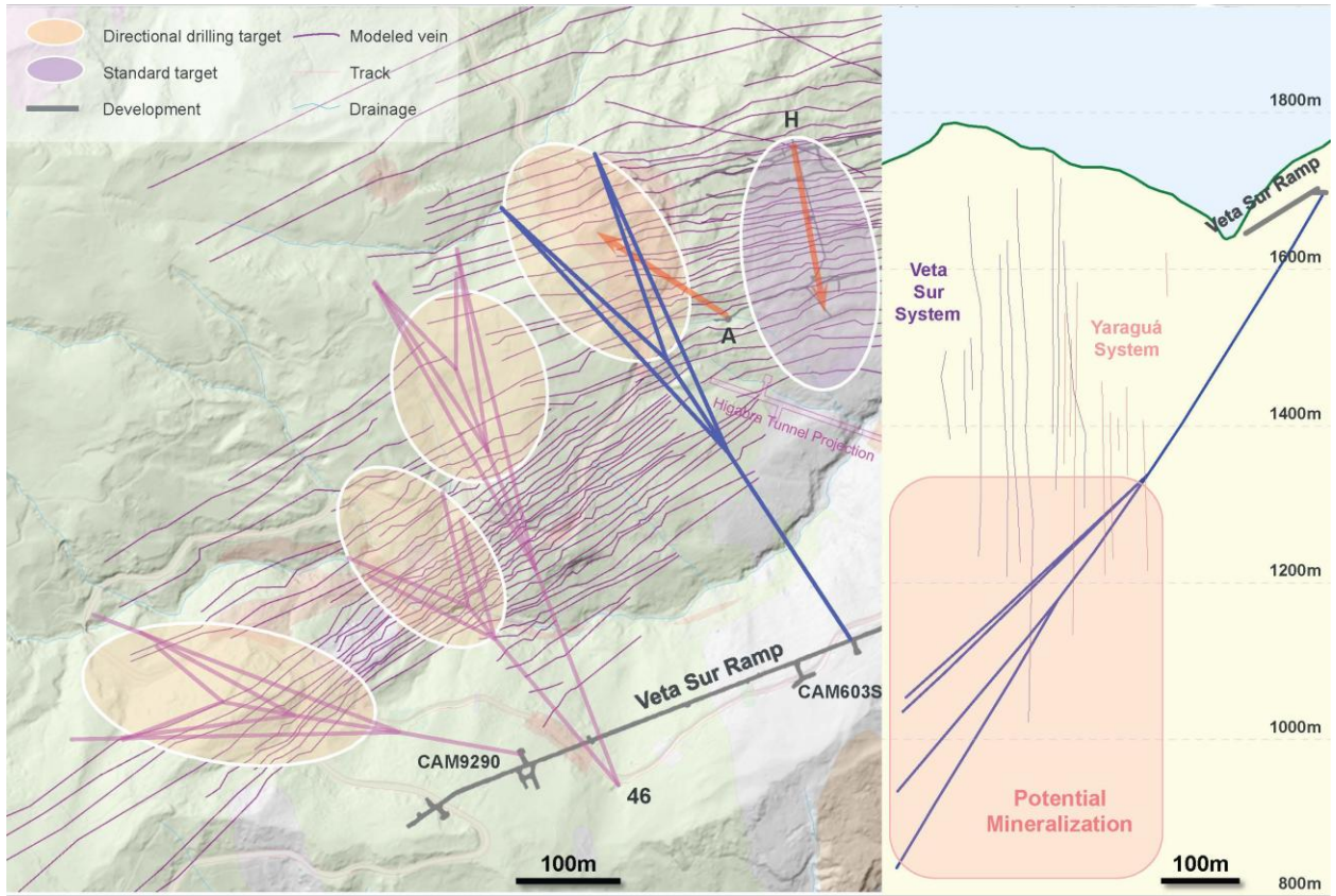
Figure 2A: Directional Drilling – Platform CAM603S
