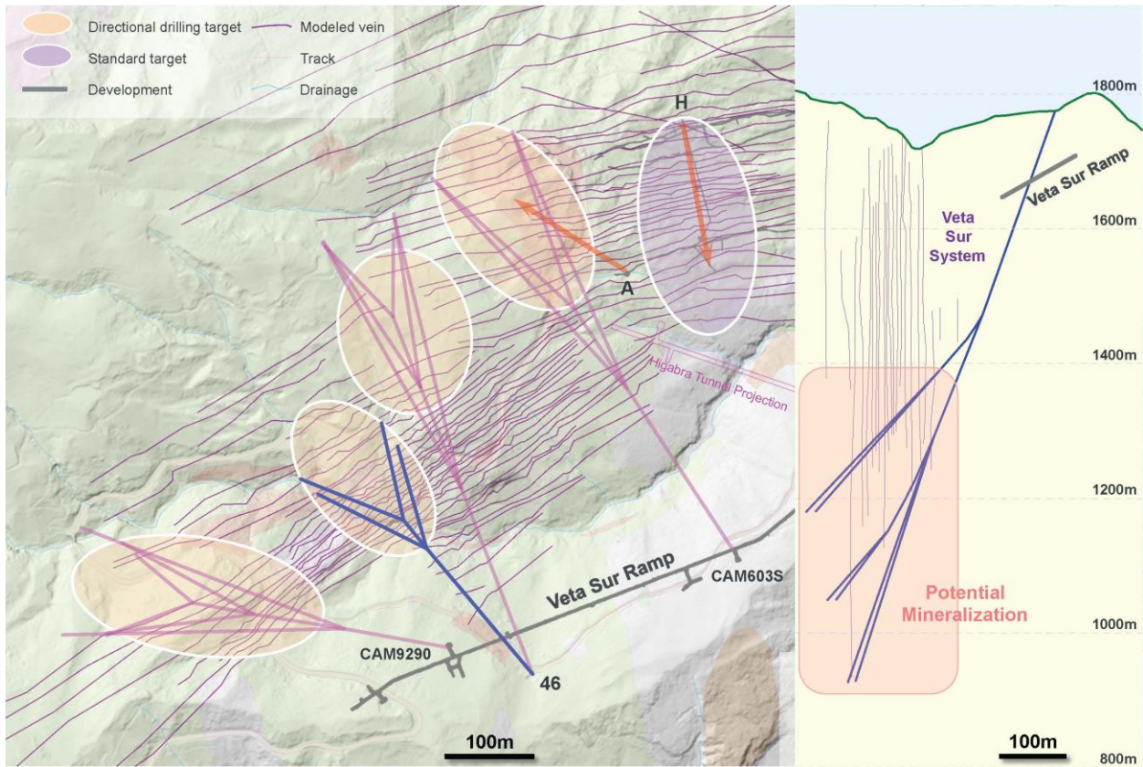
Figure 2B: Directional Drilling – Platform 46
