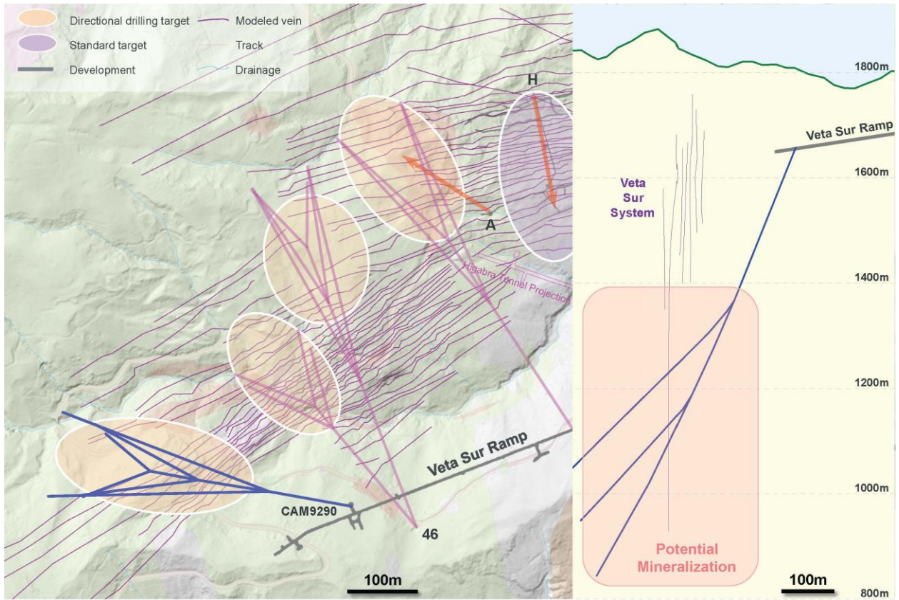
Figure 2C: Directional Drilling – Platform CAM9290
