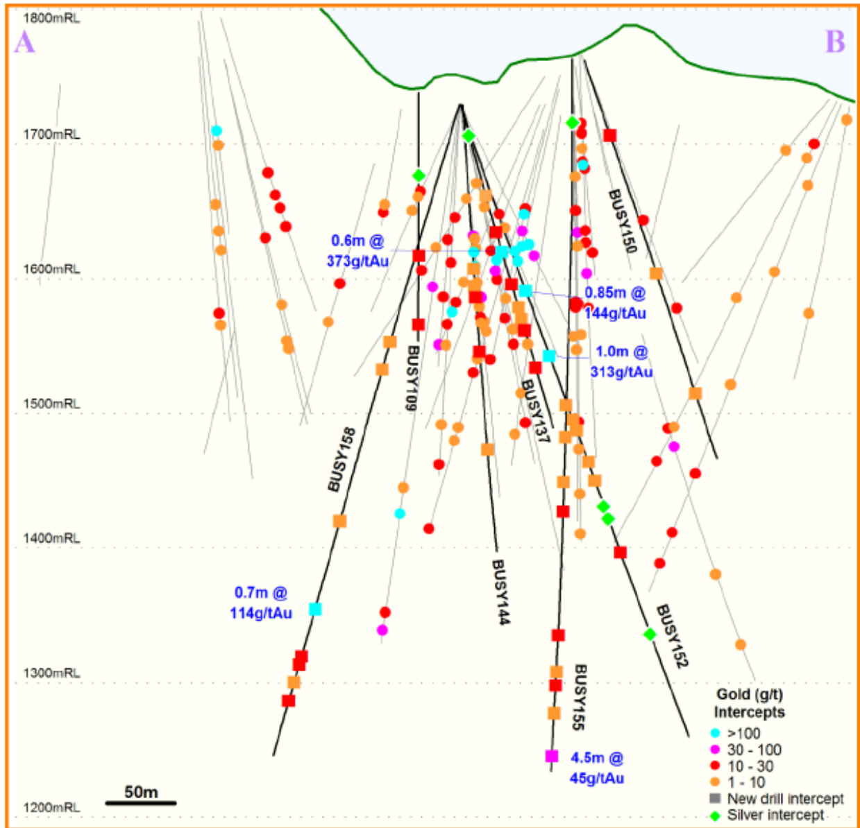
Figure 1 – Longitudinal Section of Veta Sur System
