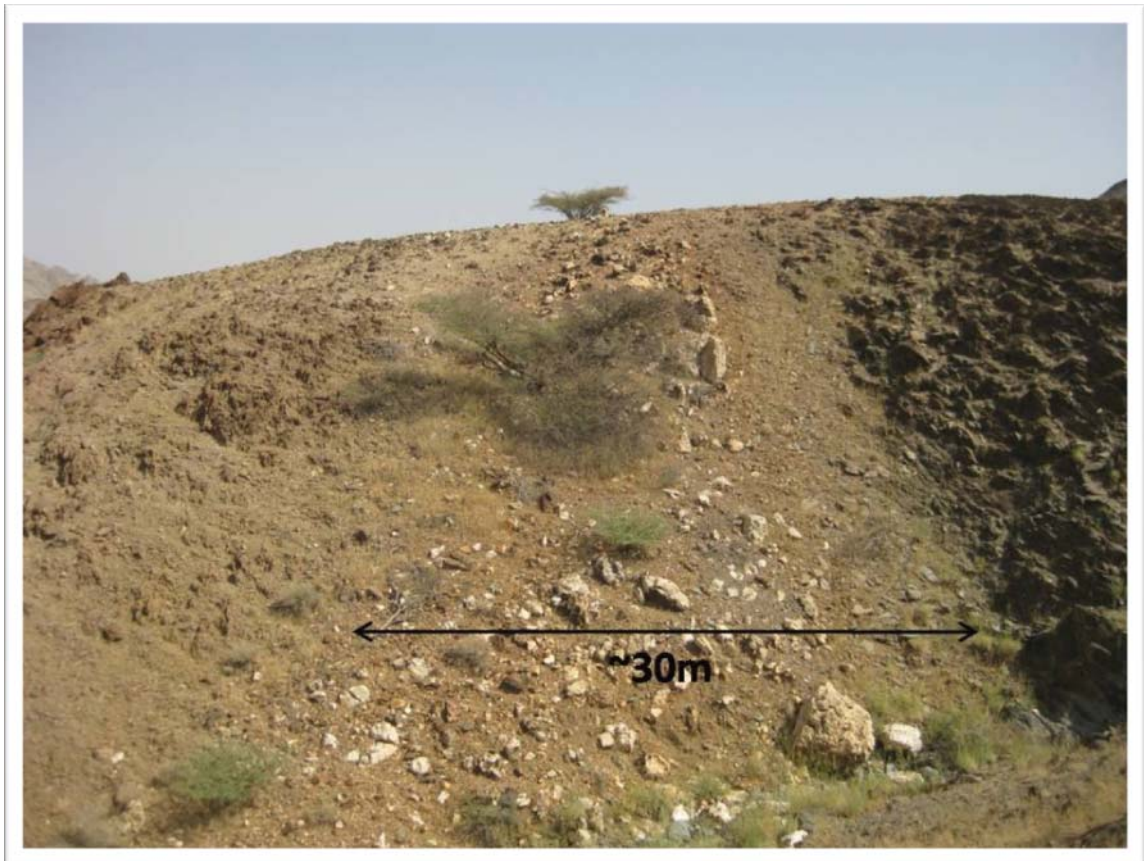
Figure 2: Zara North prospect – carbonate-sericite alteration associated with veining in source area of BLEG and conventional -80 mesh drainage geochemistry gold anomalism
