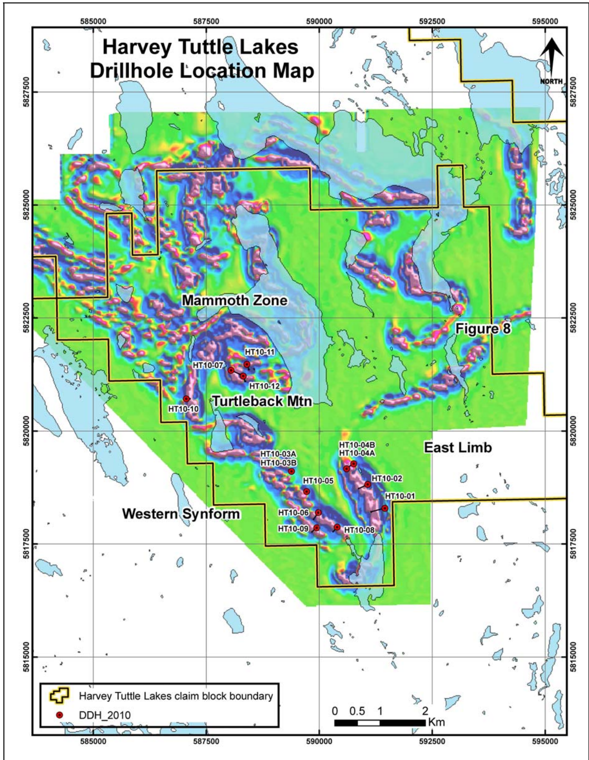
High Resolution Airborne Magnetic survey map showing the location of the Winter 2010 diamond drill holes for the Harvey-Tuttle Claim Block, Fermont Iron Property.
