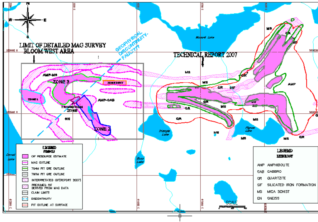
Figure 4 The geological and ore outlines prepared for the studies of the pit area with the mineralized zones (OIF) drilled to-date in the west part as well as the outlines of the magnetic survey done in 2008.
