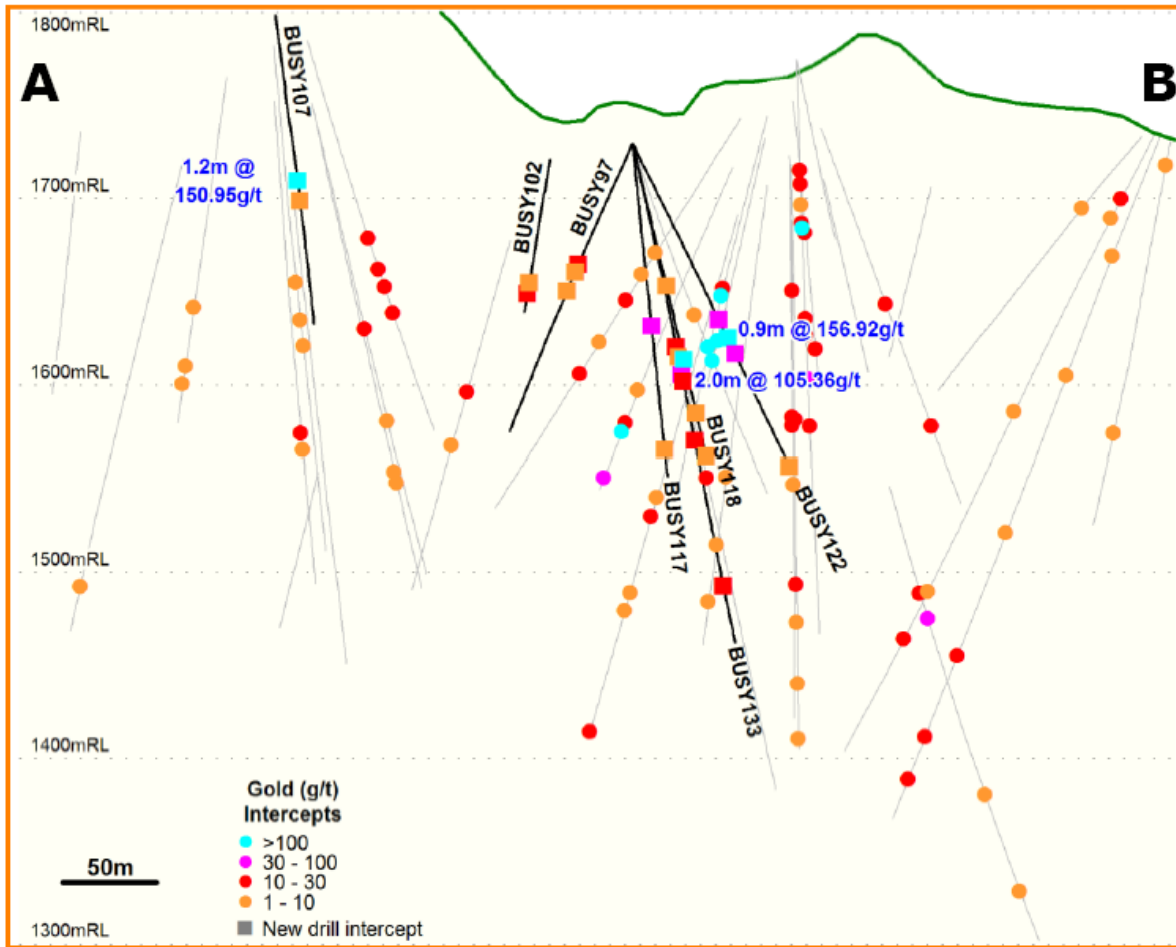
Figure 2. Veta Sur System Longitudinal Section
