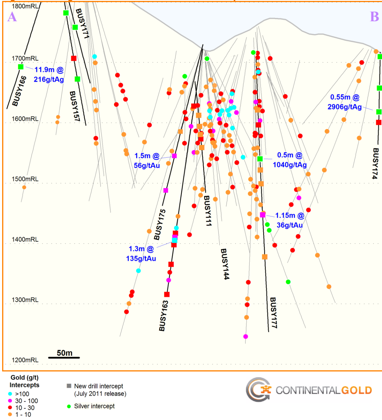
Figure 2 – Longitudinal Section of the Veta Sur Sequence
