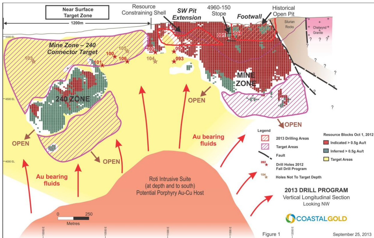
FIGURE 1: VERTICAL LONGITUDINAL SECTION
