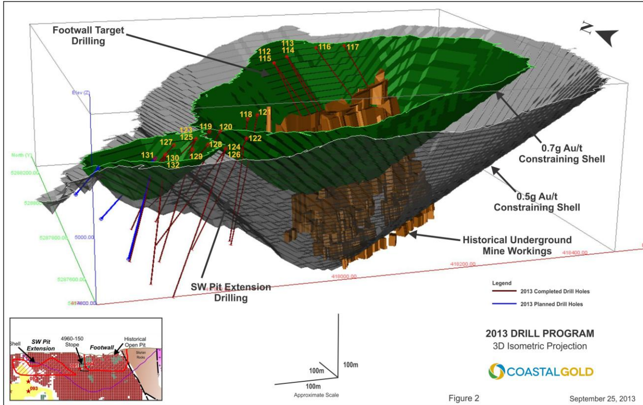
FIGURE 2: 3D ISOMETRIC PROJECTION
