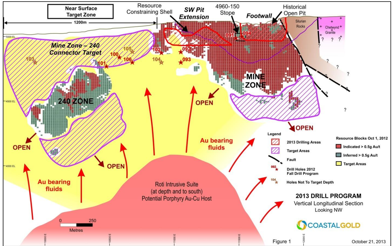
FIGURE 1: VERTICAL LONGITUDINAL SECTION
