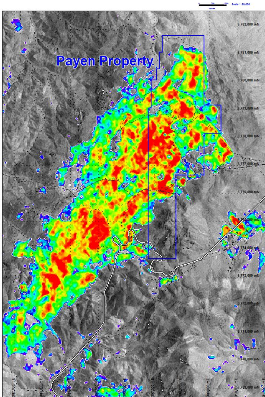
Figure 2: Pajonales alteration zone (clay intensity), Payen property boundary and Panamerican Highway
