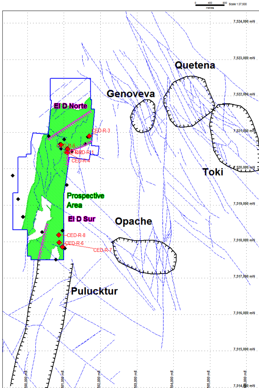
Figure 1: El Desesperado Location, showing Coro claim block in blue, Toki Cluster deposits in black hachured lines, Coro RC holes in red, old holes in black, prospective area in green, target areas in pink, faults in blue.
