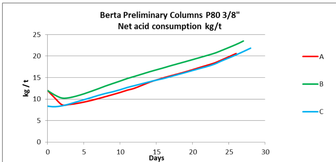
Figure 2: Berta net acid consumption
