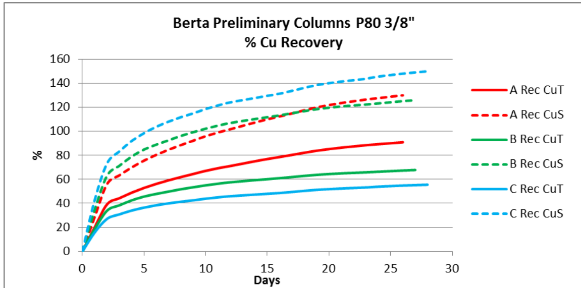
Figure 1: Berta leach kinetics
