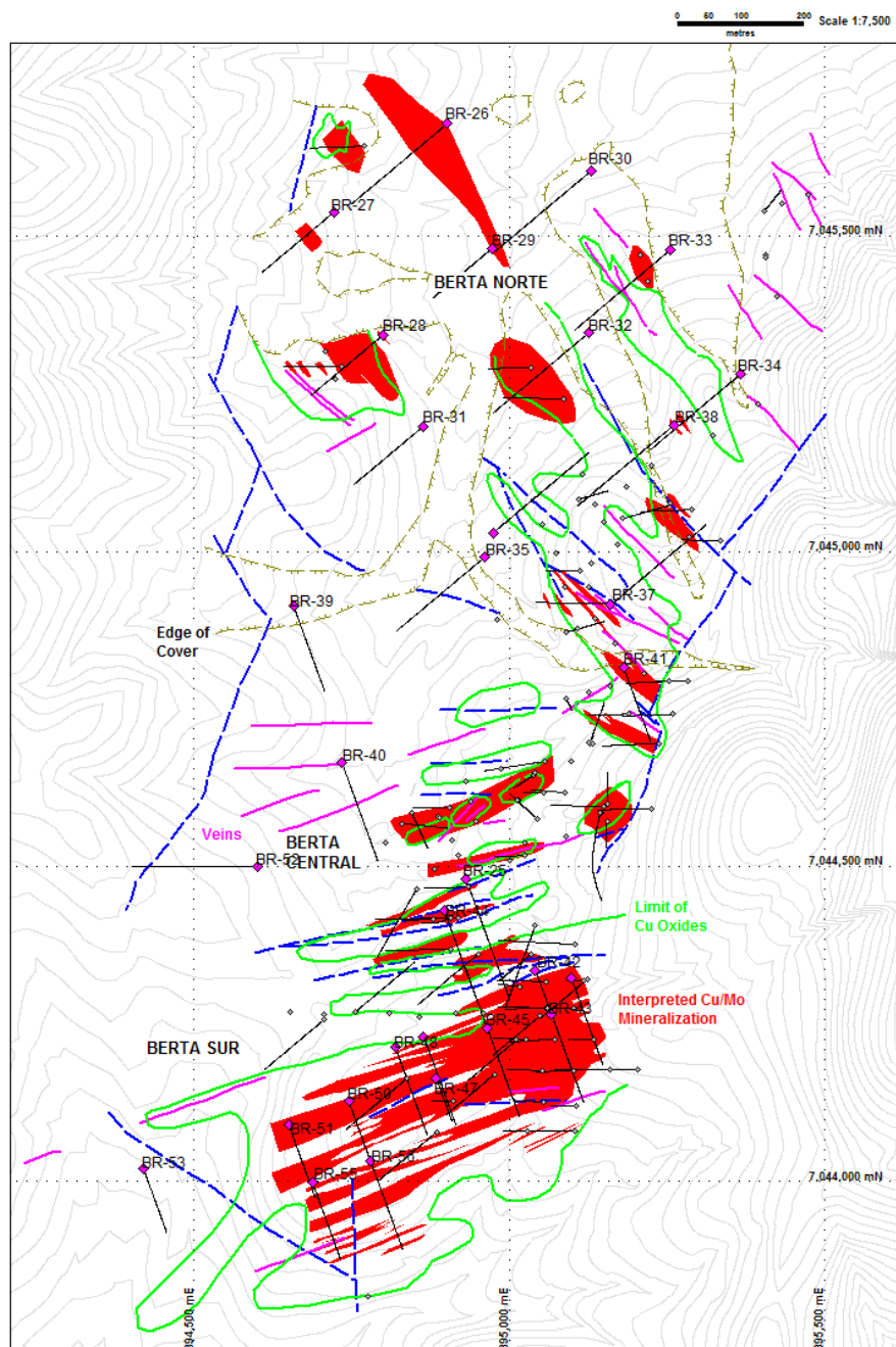
Figure 1: Drill tested copper mineralization shown in red, limit of mapped copper oxides in green, faults shown in blue, Cu bearing veins in pink, Coro RC hole collars in pink.
