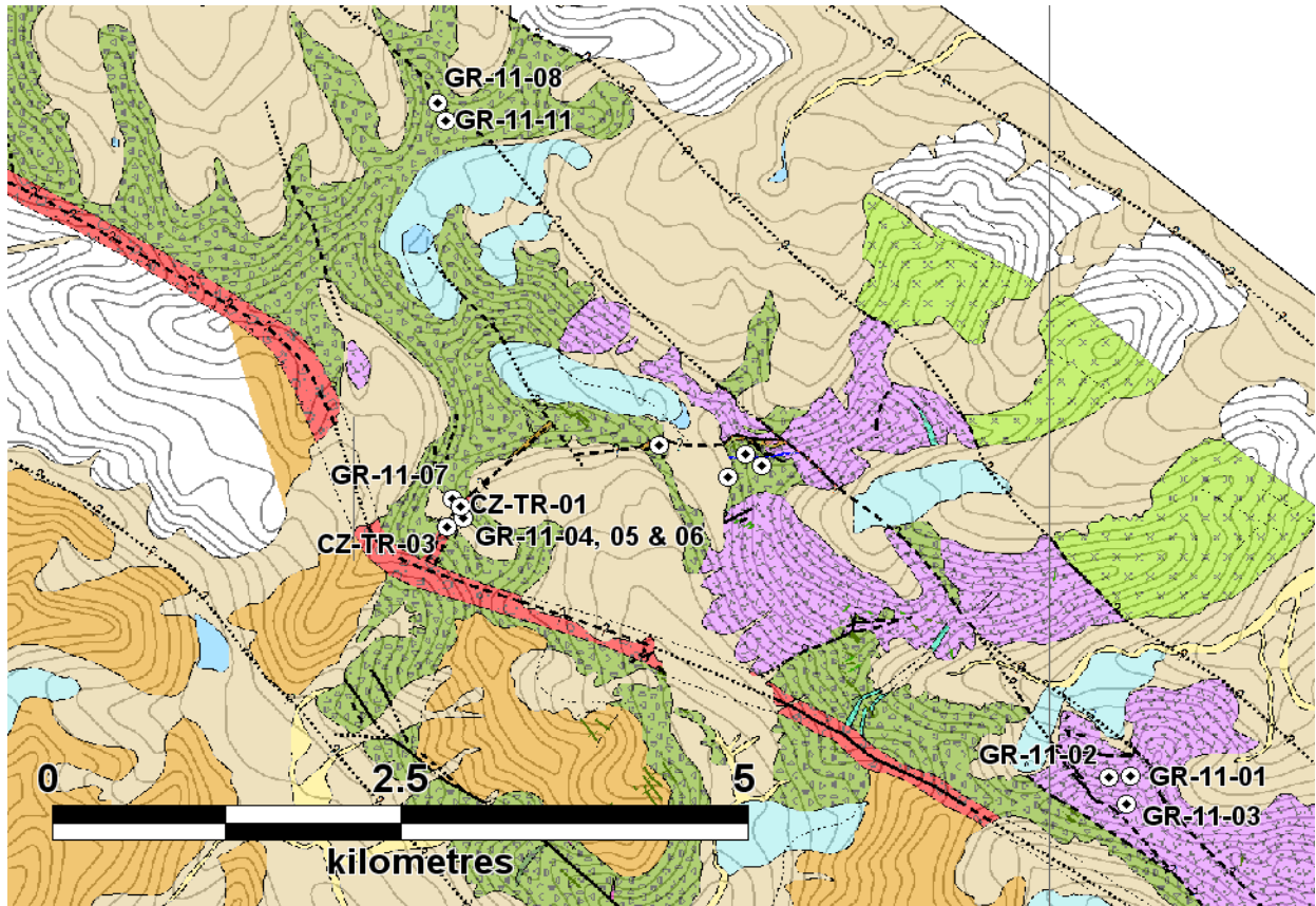
Figure 2: Geological map of central Golden Range showing the locations of hole collars at Corazon, Matador and City reported in this press release.
