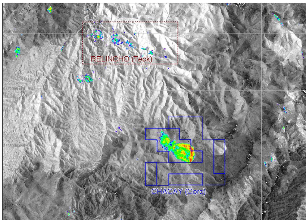
Figure 1: Location Map (Chacay Property; MCAL exploitation claims shown with thick blue line, exploration claims shown in thin blue line. Clay alteration from satellite imagery) (10km Grid)
