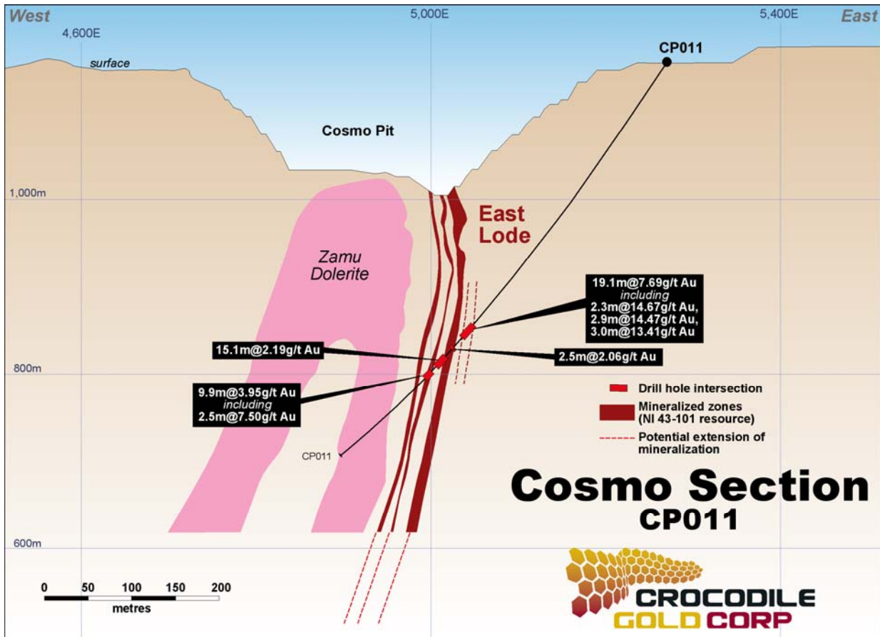
Figure 4: Cosmo Section – Hole CP011
