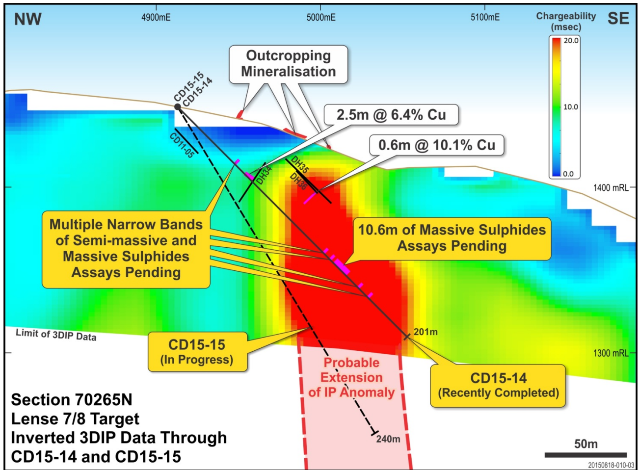
Figure 1. Cross section of inverted 3DIP data through the underexplored Lense 7/8 Target, illustrating shallow high-grade mineralisation intersected in previous drilling together with the location of massive sulphides intersected in the recently completed drill hole CD15-14, and the intended projection of follow-up drill hole CD15-15, which is currently in progress.
