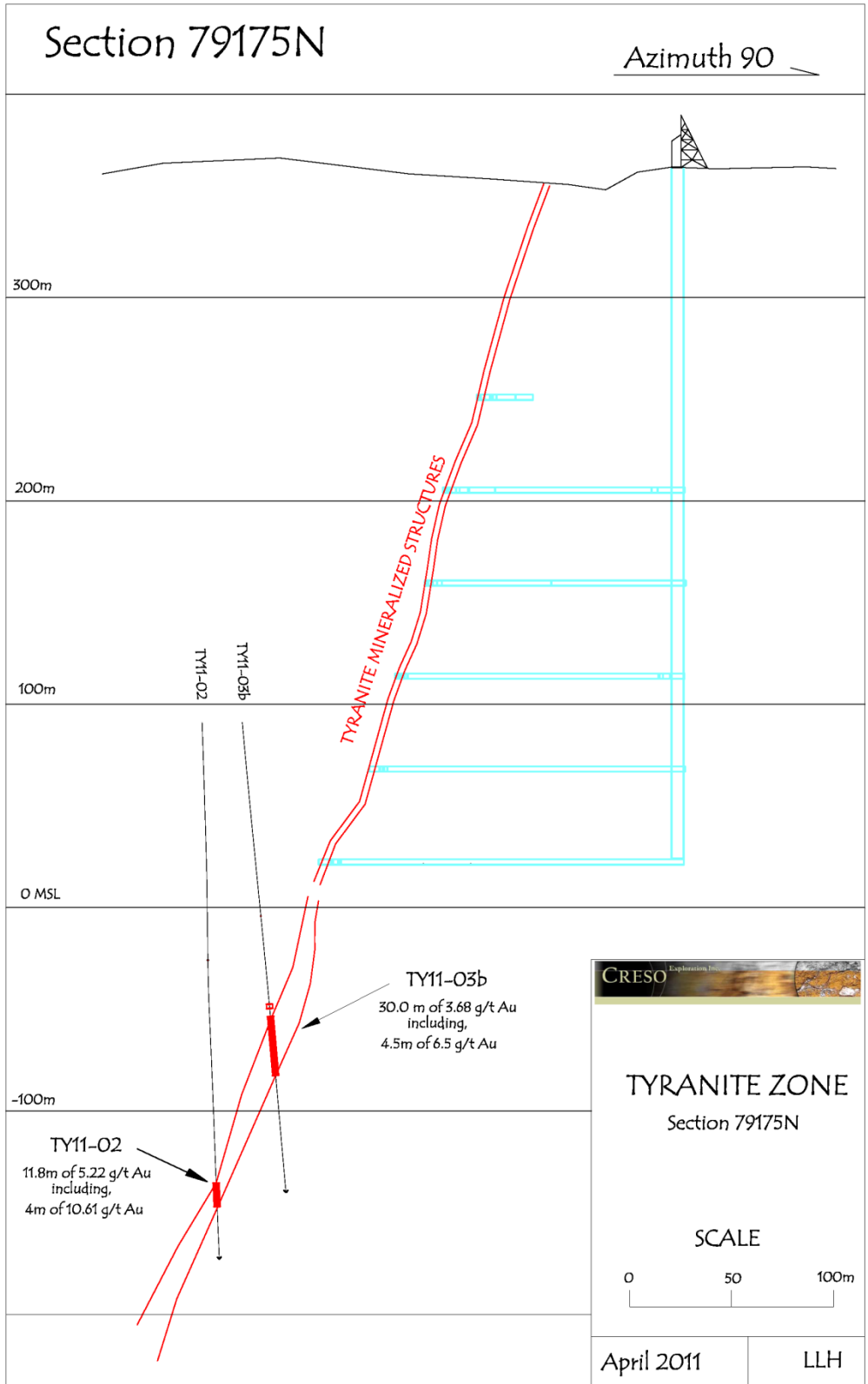
Figure 3. Cross-Section 79175N at the Tyrannite Zone, Ontario
