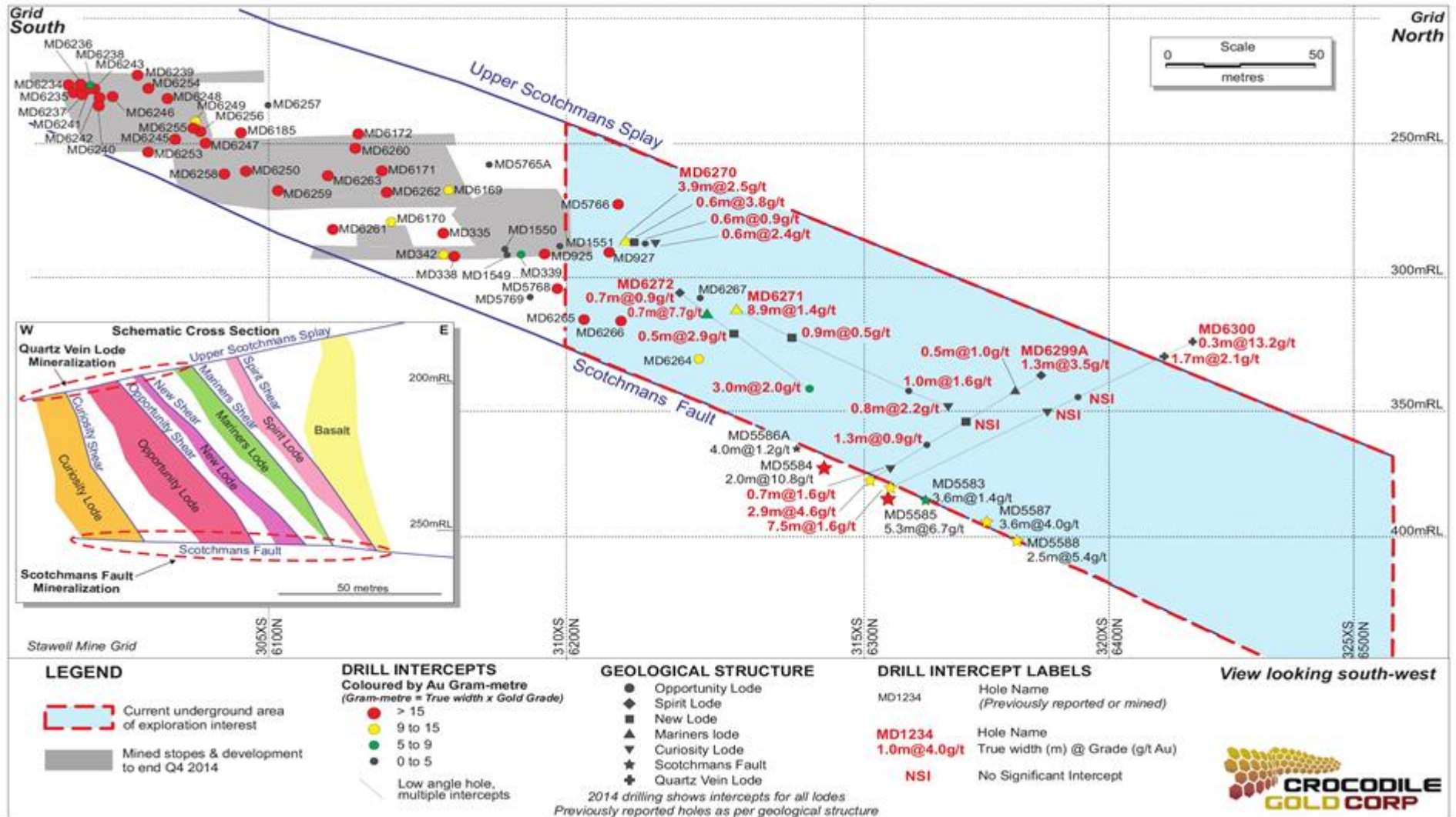
Figure 6: Mariners Longitudinal Projection, Opportunity Lode, Stawell Gold Mines
