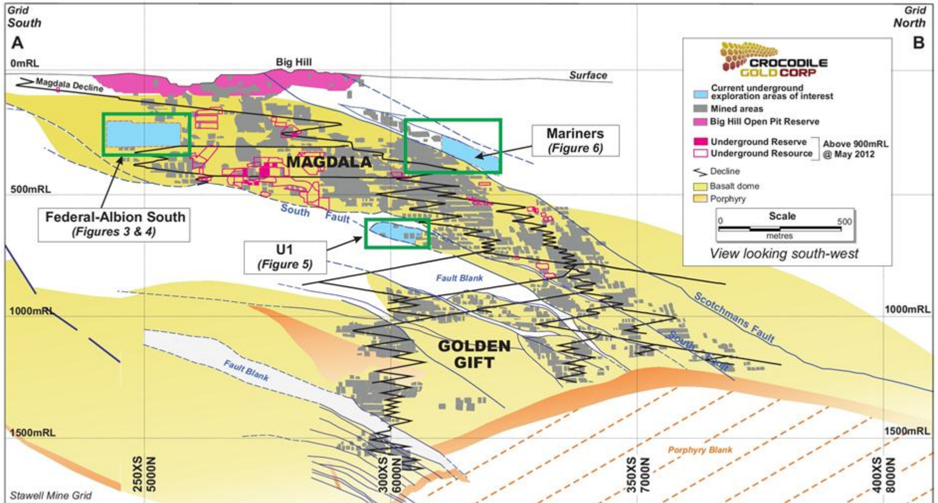
Figure 2: Longitudinal Projection, Magdala Mine, Stawell Gold Mines
