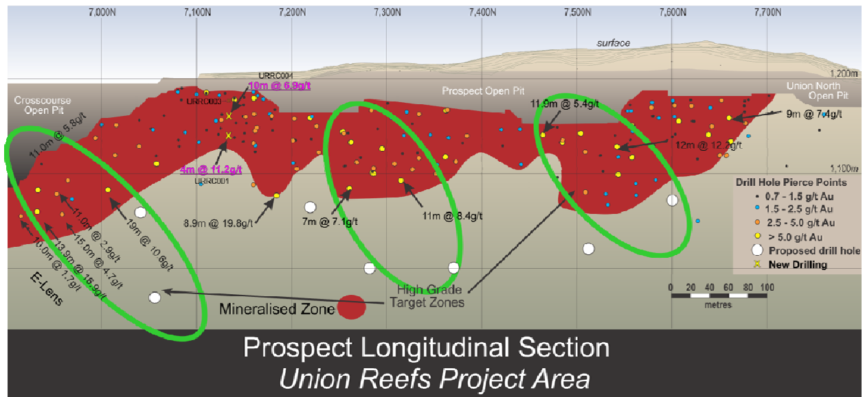
Figure 4: Prospect Longitudinal Section (looking west) (Image shows Union Mineralized Zone which contains the E-Lens Mineralization in Crosscourse)
