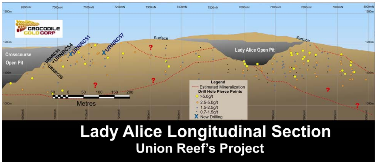
Figure 4: Longitudinal Section of Lady Alice Deposit on Lady Alice Mineralized Zone showing latest drilling
