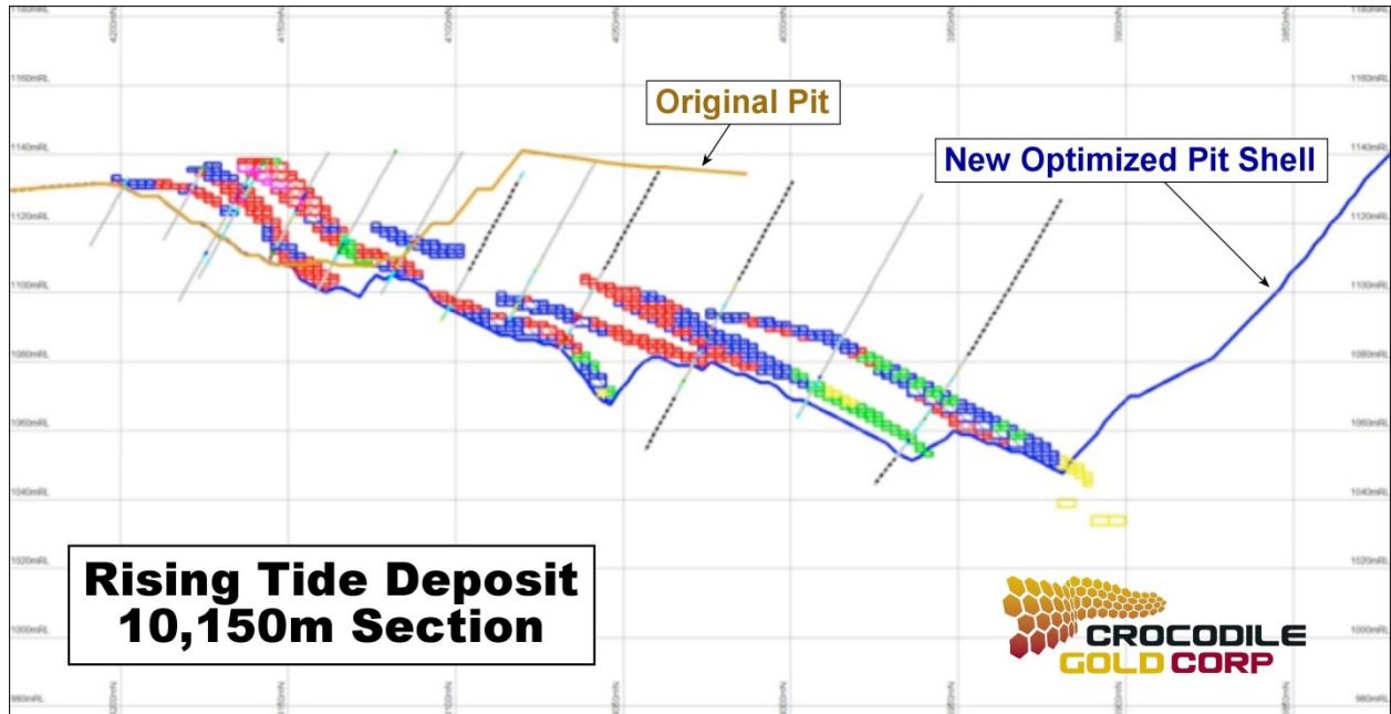
Figure 4: Cross Section of Rising Tide Optimized Pit Shell
