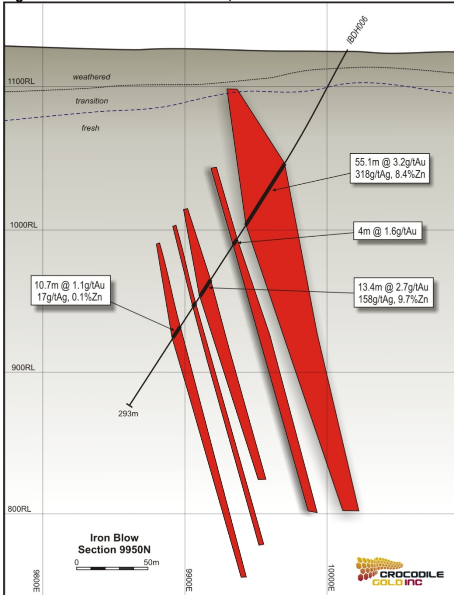
Figure 6: Iron Blow Cross Section 9,950N
