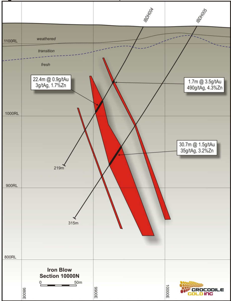
Figure 5: Iron Blow Cross Section 10,000N
