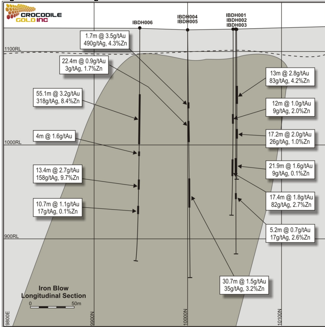
Figure 3: Iron Blow Longitudinal Section
