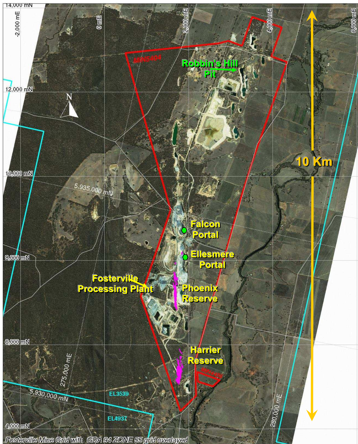
Figure 1: Fosterville Gold Mine Site Plan
