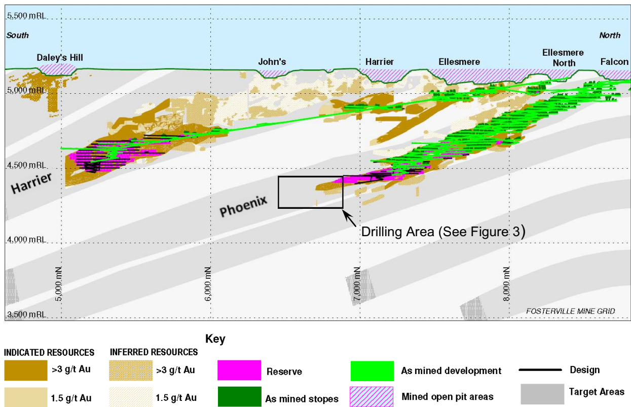
Figure 2: Fosterville Fault Ore body Long Projection
