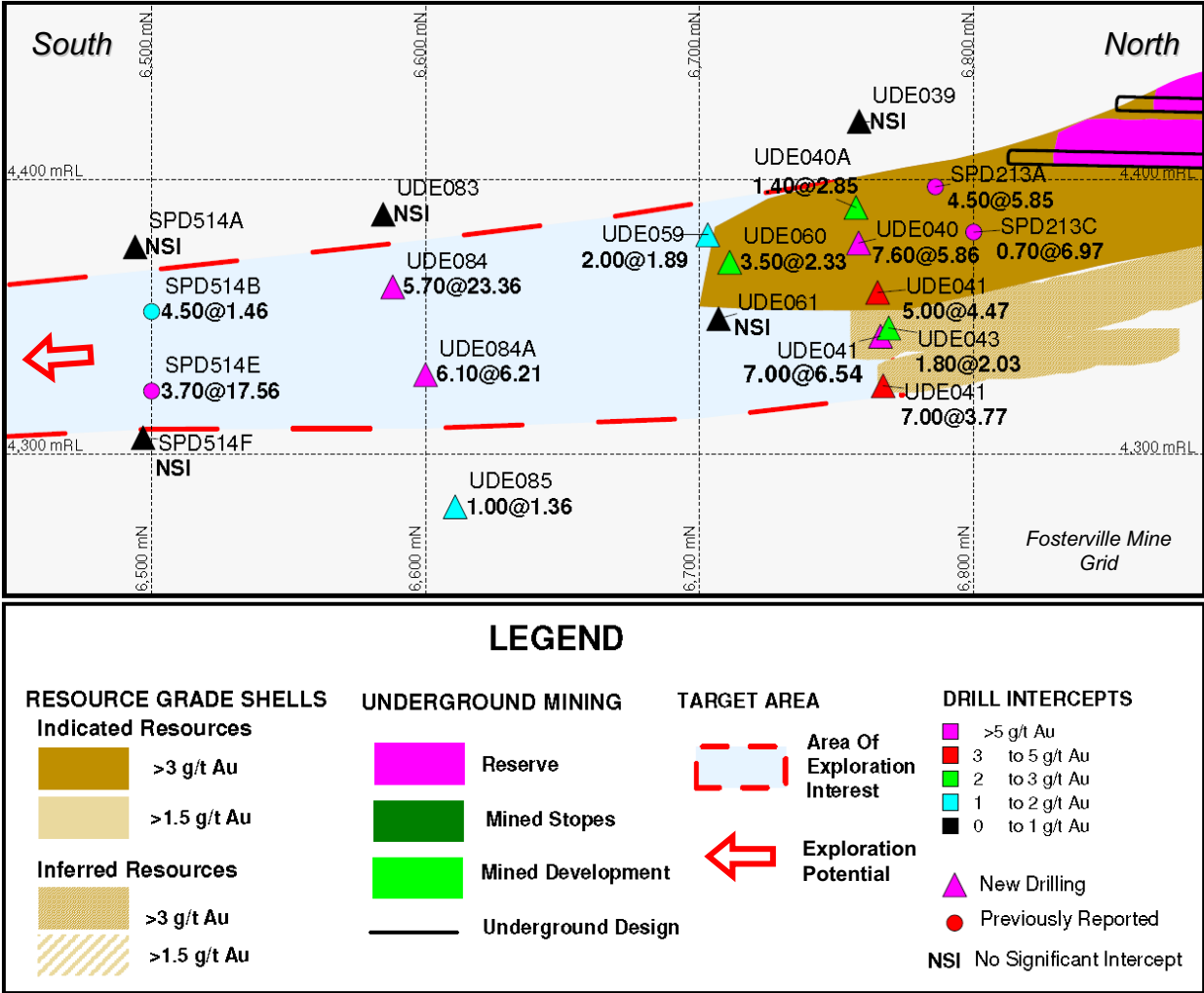
Figure 3: Phoenix Long Projection
