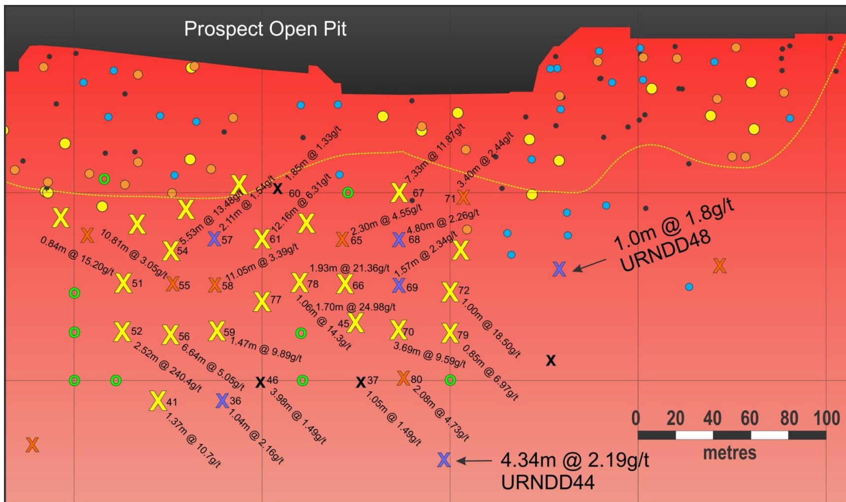
Figure 4: Close up of Area of Detailed Drilling, Prospect Deposit
