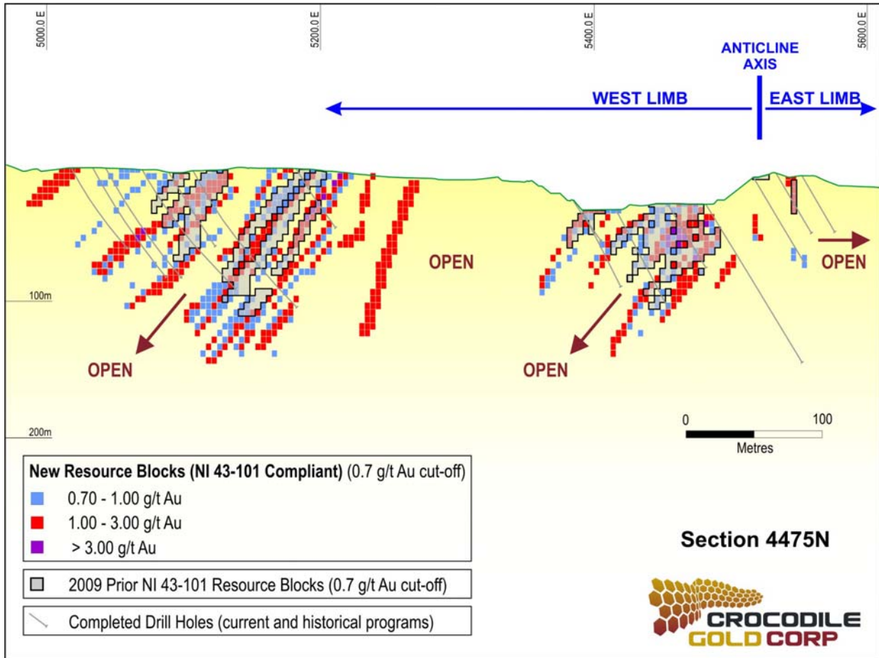
Figure 3: Representative Cross Section (4475N) showing comparison of updated to previously announced resources
