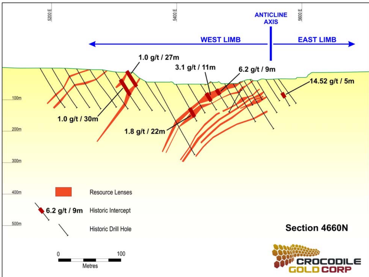
Figure 4: Composite Cross Section of Chinese showing resource blocks
