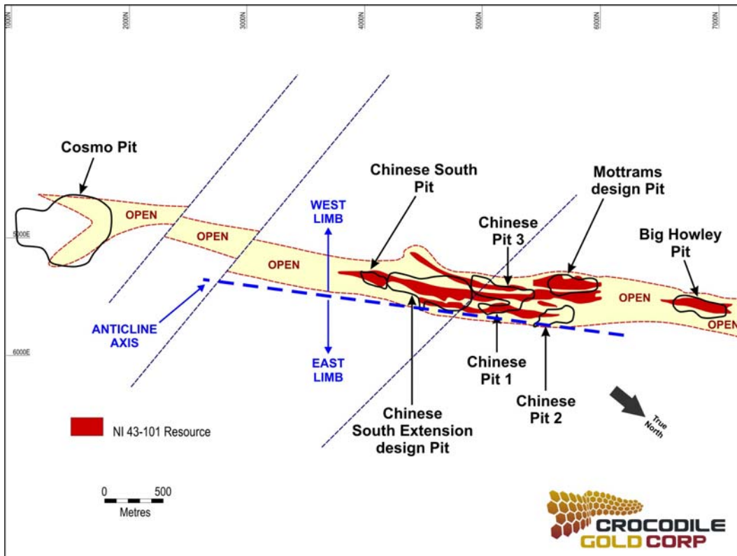
Figure 2: Chinese Plan View
