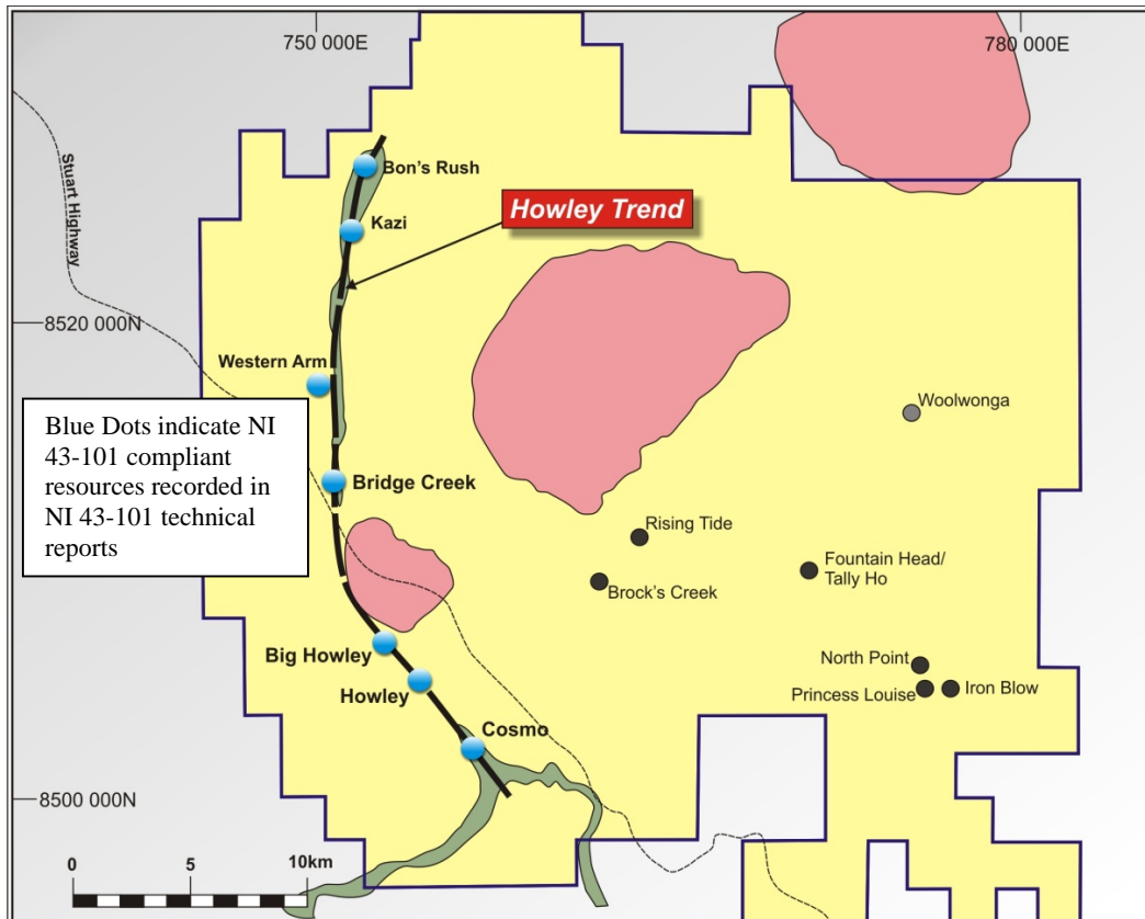
Figure 2: Mineralization Along Howley Trend
