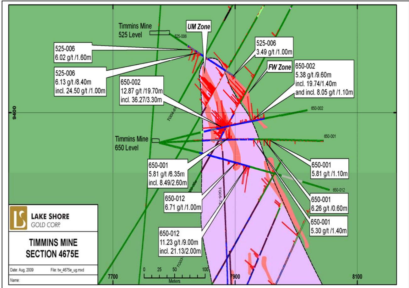
Figure 2. Cross Section
