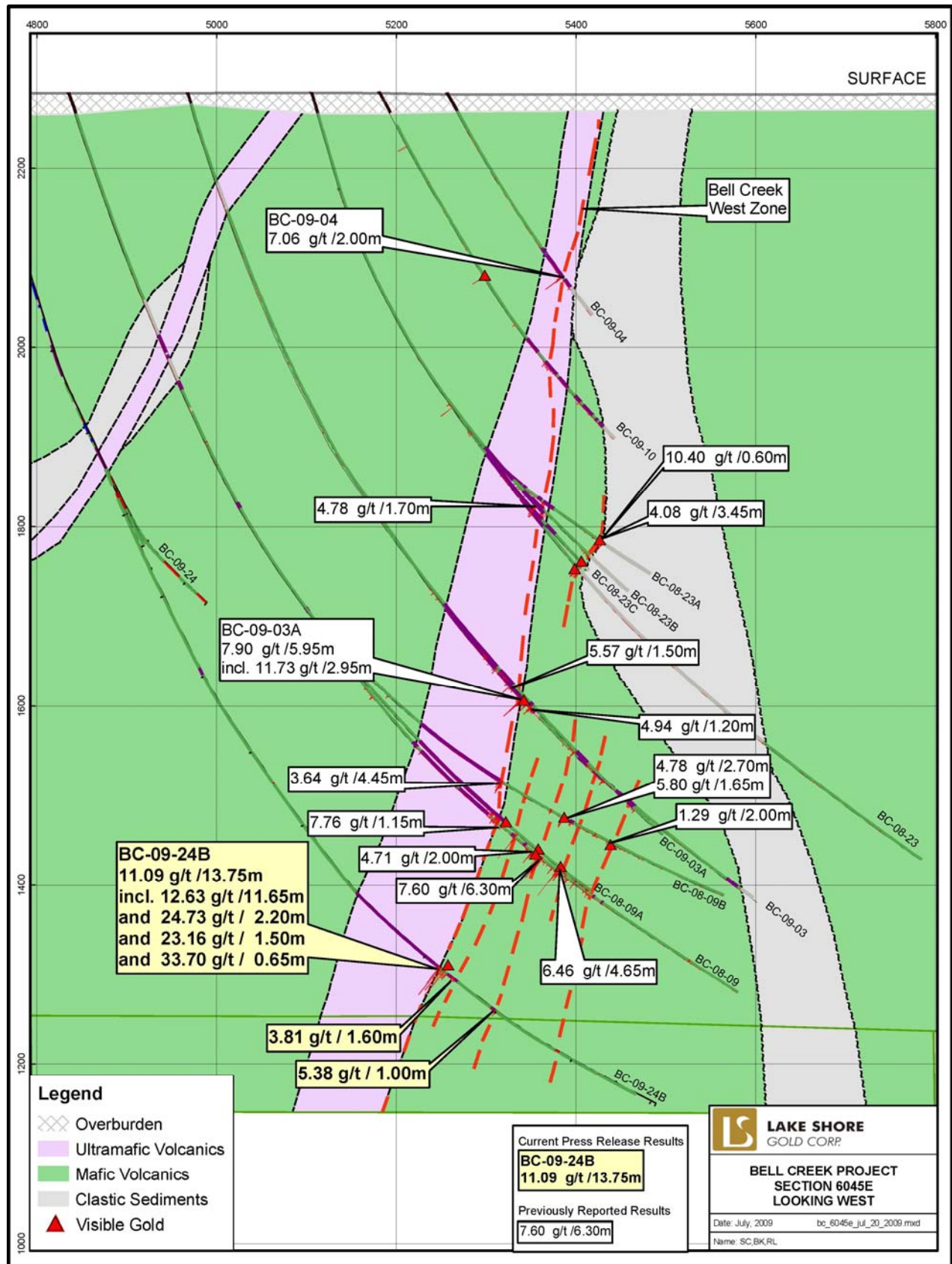
Figure 2. Cross Section
