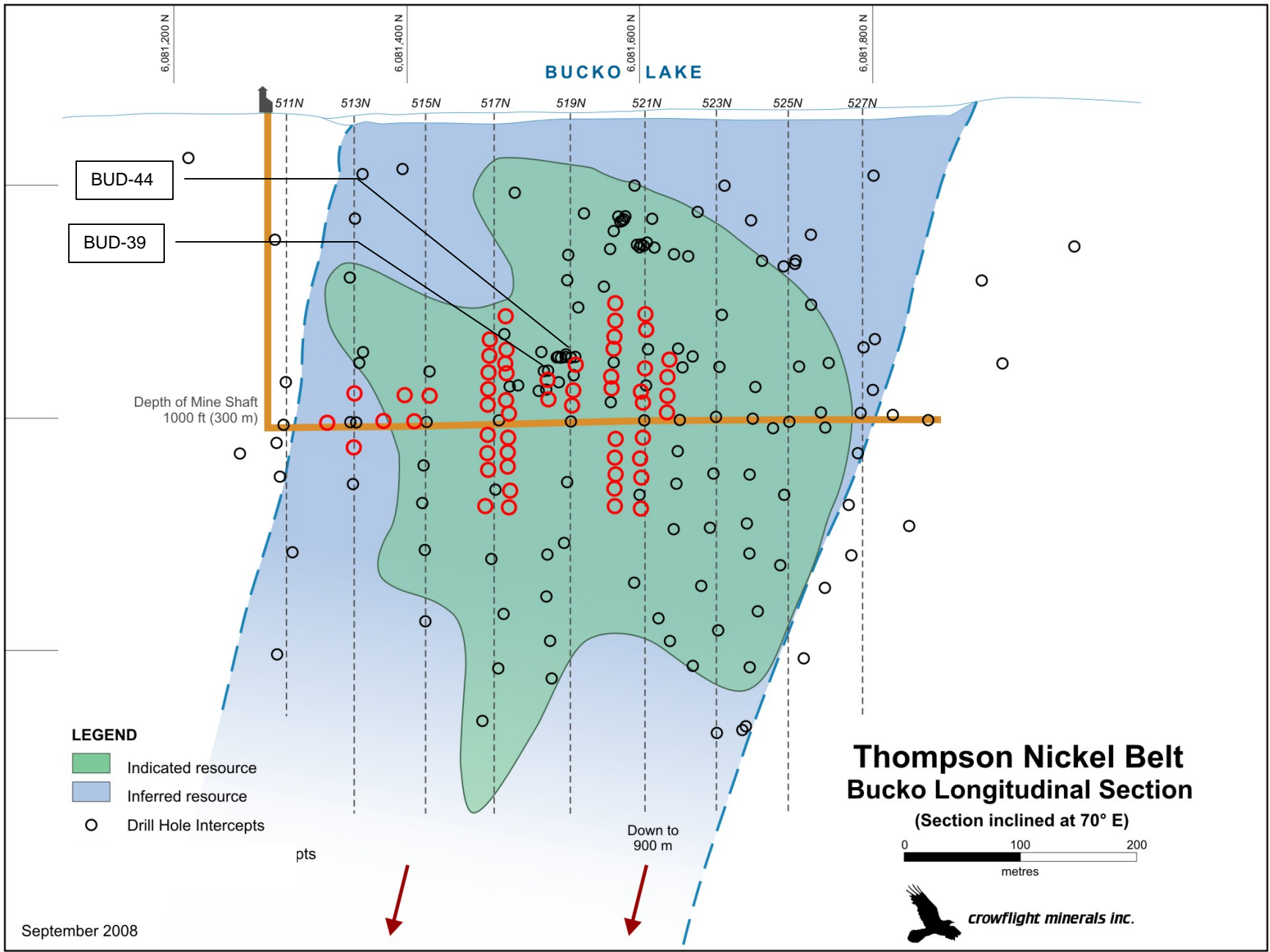
Figure 1. Assay Results from 1,000 Foot Level Delineation Program
