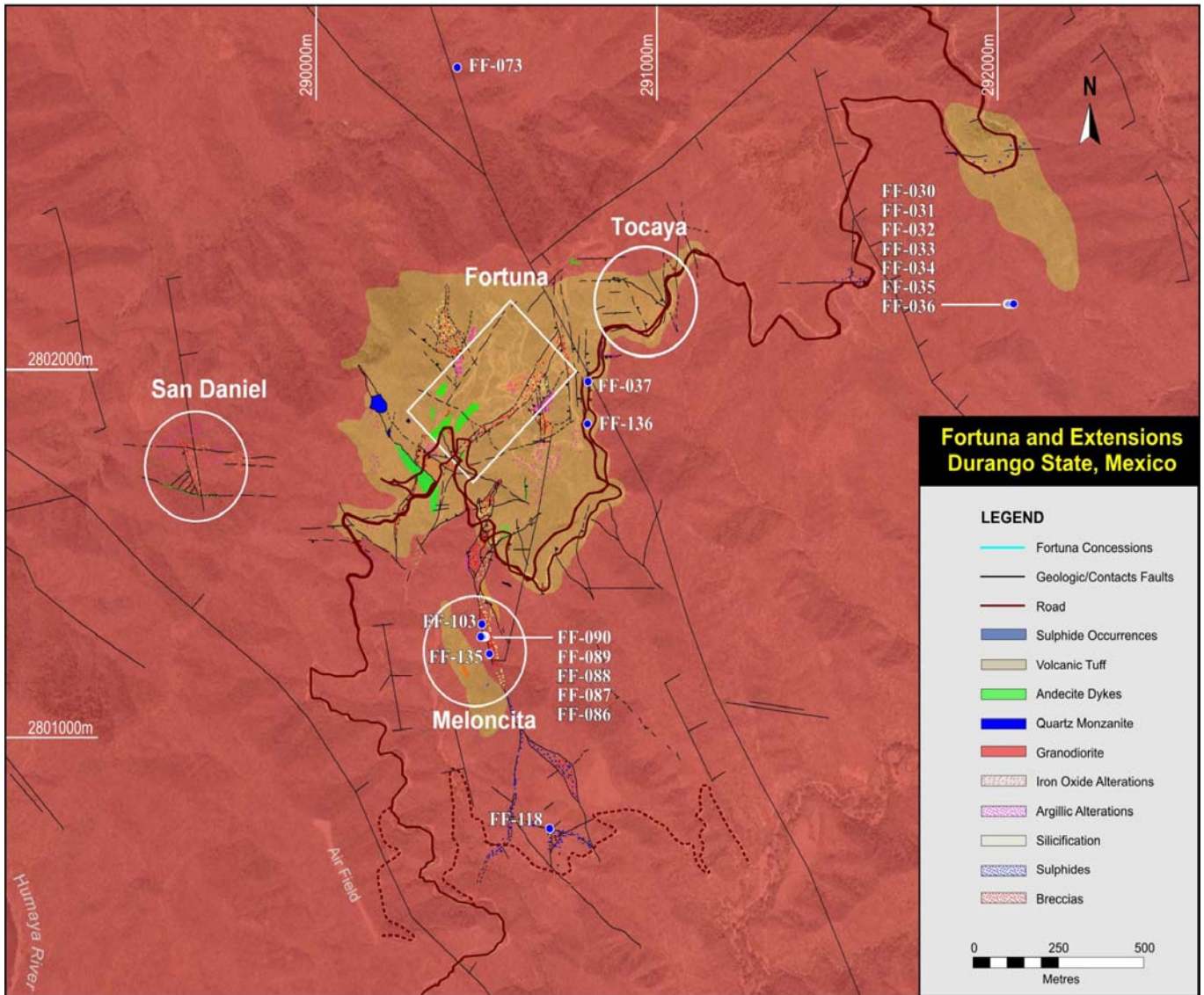
Image 2 La Fortuna and Extensions Geologic and Sample Location Map
