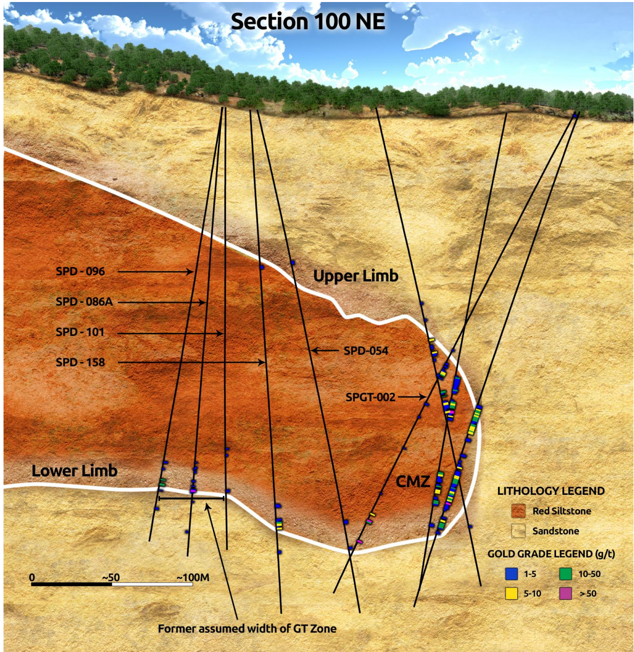
Figure 3: Cross-Section of 100NE
