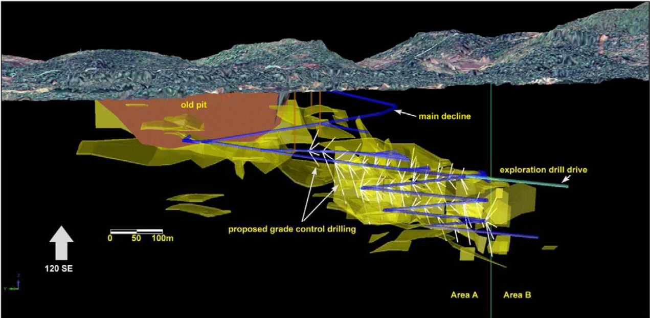
Figure 1: Proposed Underground Development
