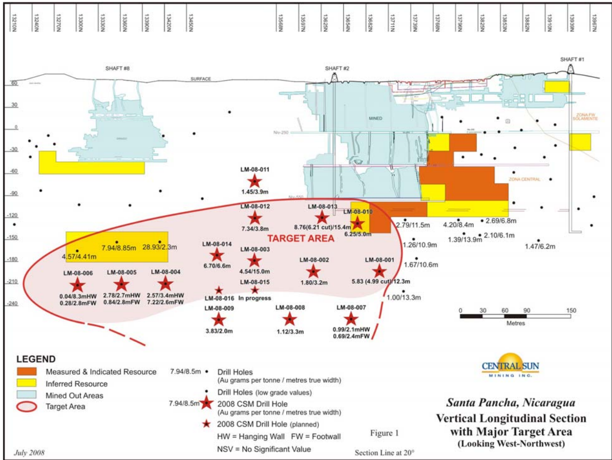
Figure 1: Limon Mine, Santa Pancha vertical longitudinal section
