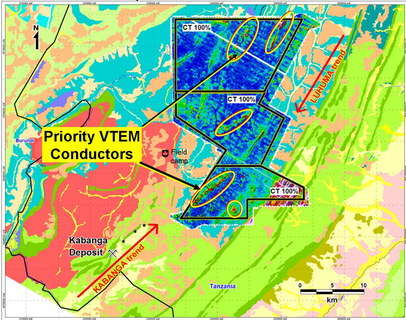
Figure 2: Kagera VTEM anomalies on Regional Geologic map showing the location of the Kabanga nickel sulfide deposits to the south and the Luhuma nickel occurrences to the northeast of the Castilian survey area.
