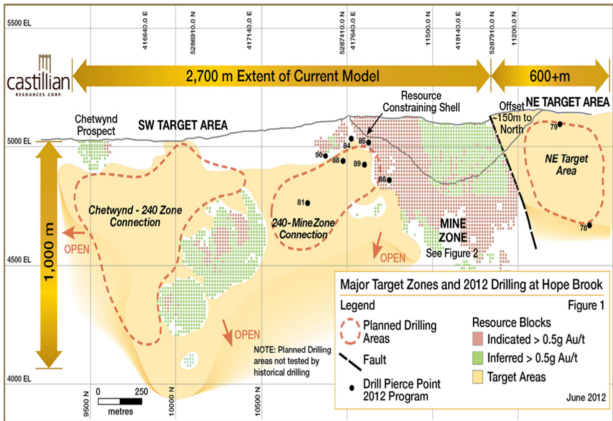
Figure 1: Longitudinal Section with location of pierce points for drilling the Southwest and Northeast Target Areas (see Figure 2 for drilling in Mine Zone area).
