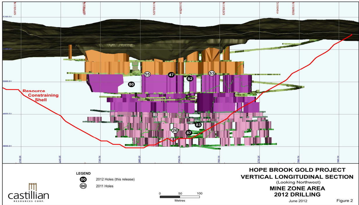
Figure 2. Longitudinal Section of Mine Zone area showing locations of drill hole pierce points
