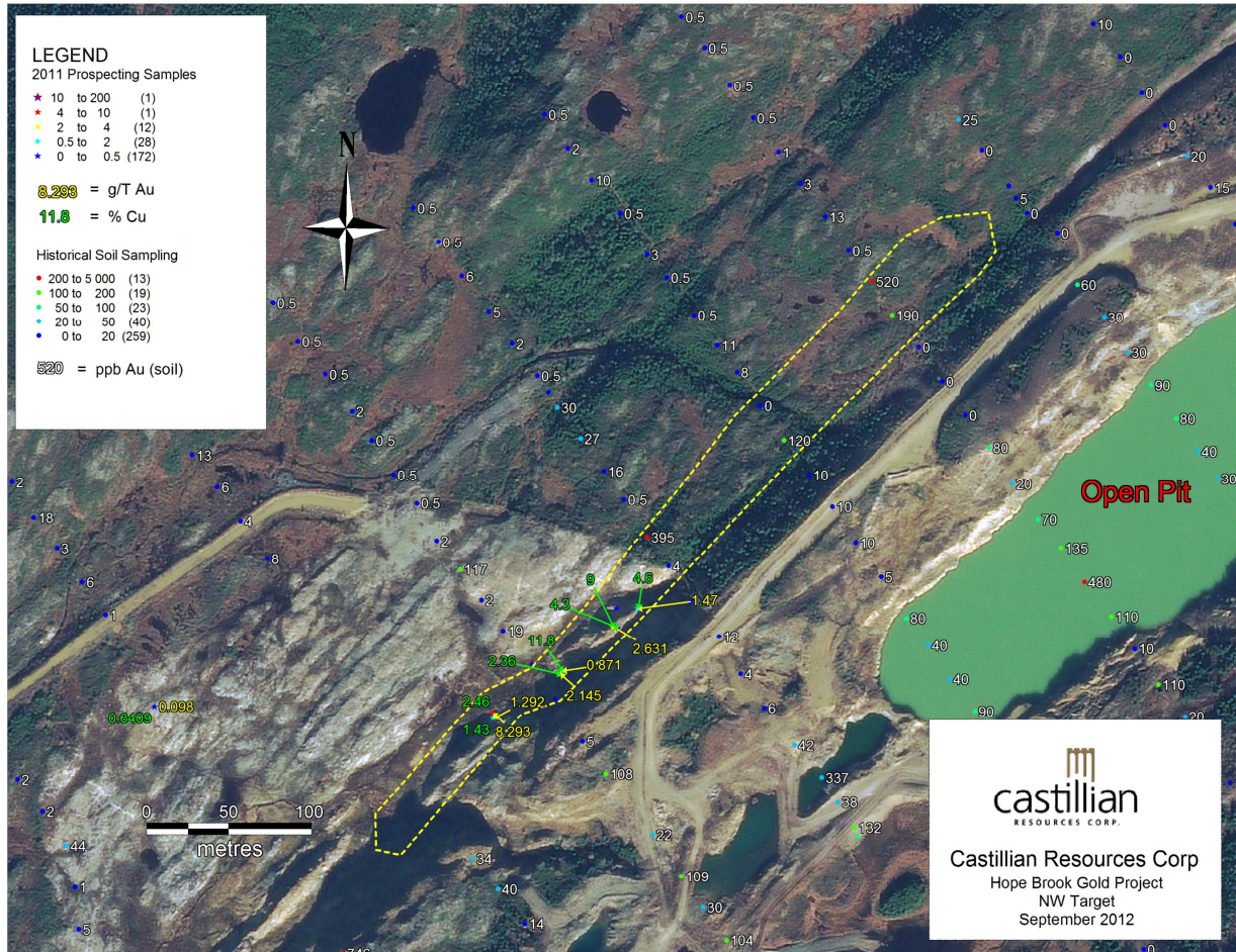
Figure 3. Plan Map showing location of new Au-Cu target area northwest of open pit
