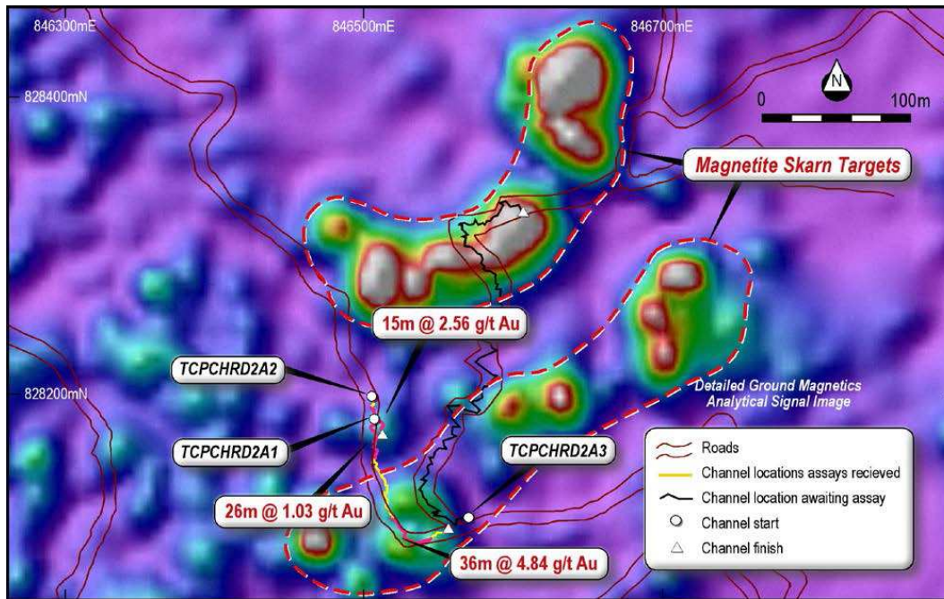
Figure 4 – Taggura North channel sample and mineralisation locations on ground magnetics analytical signal image. Hot colours indicative of magnetite skarns.
