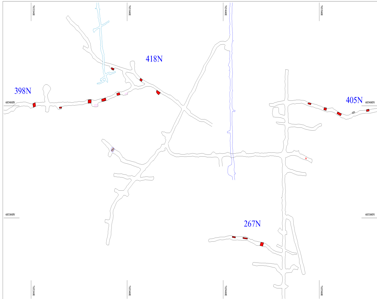
Figure 2: Underground development with existing raises shaded red (WGS84UTM)
