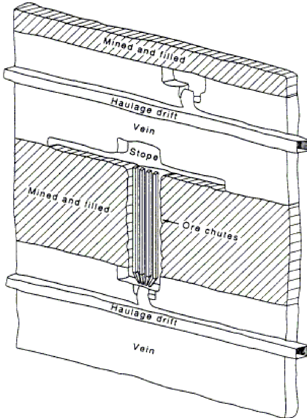
Figure 3: Example of Cut-And-Fill Mining Method
