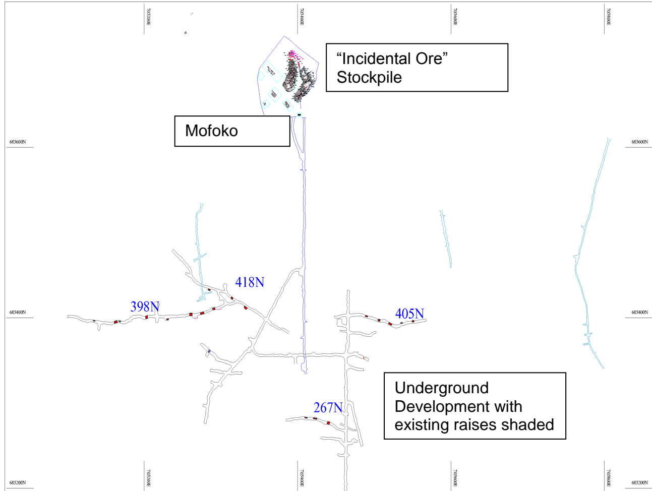
Figure 1: Underground development with existing raises shaded red and surveyed "incidental ore" stockpile (WGS84UTM)
