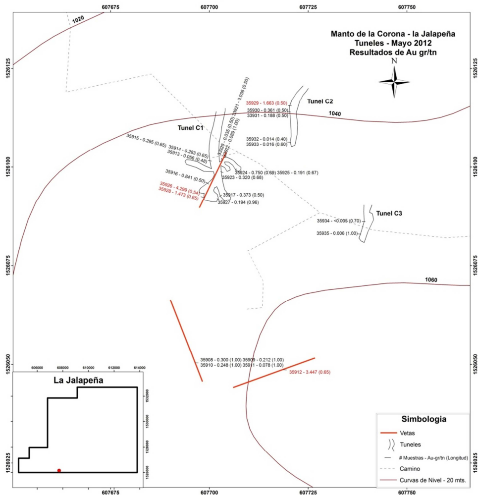
Figure 2: Manto de La Corona La Jalapeña Tunnels and Assay Results, Neuva Segovia, Nicaragua
