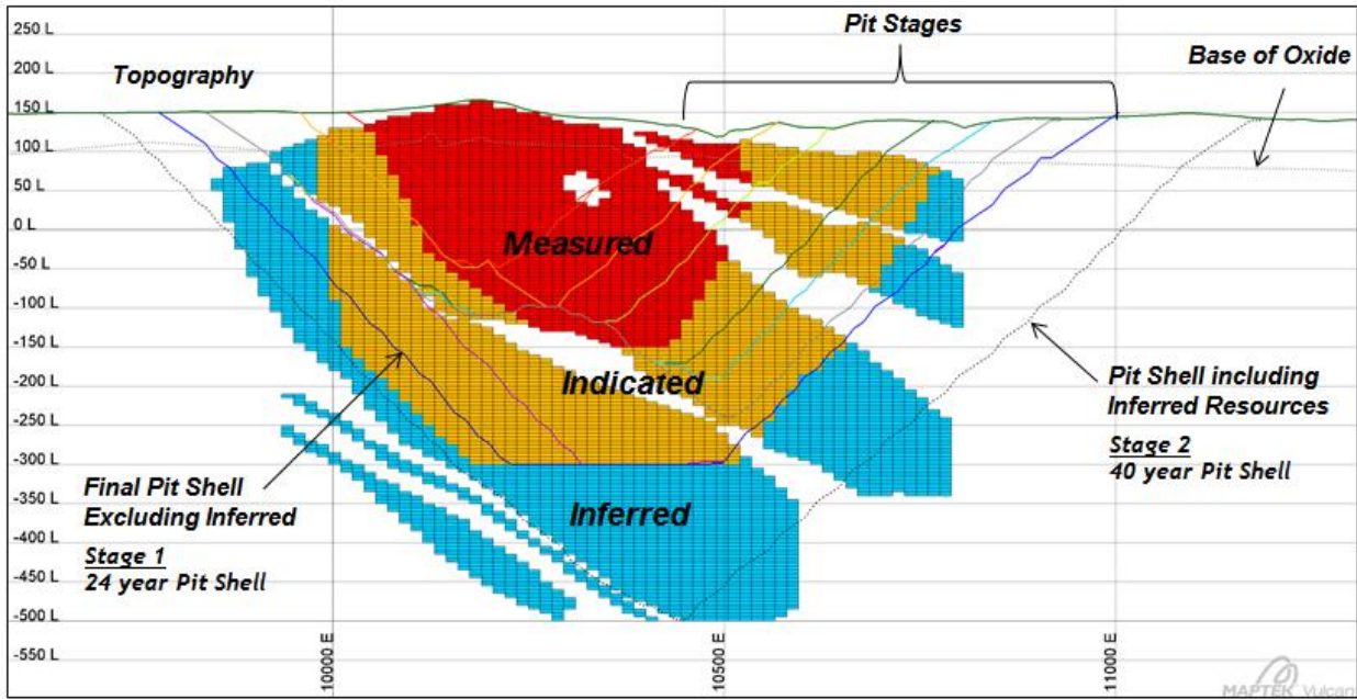
Figure: Looking North - Section 19500N (local grid): Optimized Pit Shells
