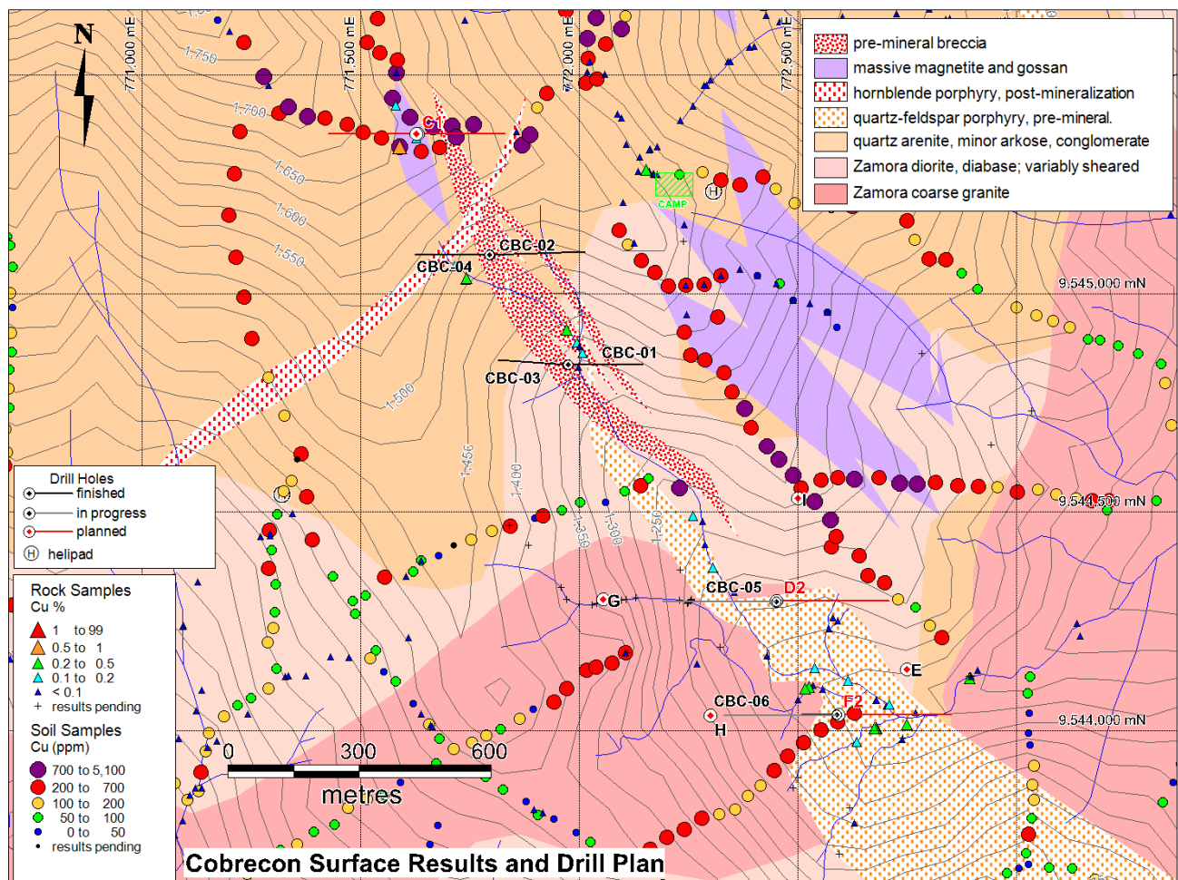
Figure 1: Cobrecon Drill Target Map. Previously reported and new soil and rock sample results. Note the numerous samples returning between 0.2 and 0.5% Copper in the area of current drilling (holes CBC-05 & CBC-06) in bottom right quarter of the map; this area is the most consistently mineralized zone discovered to date at Cobrecon.
