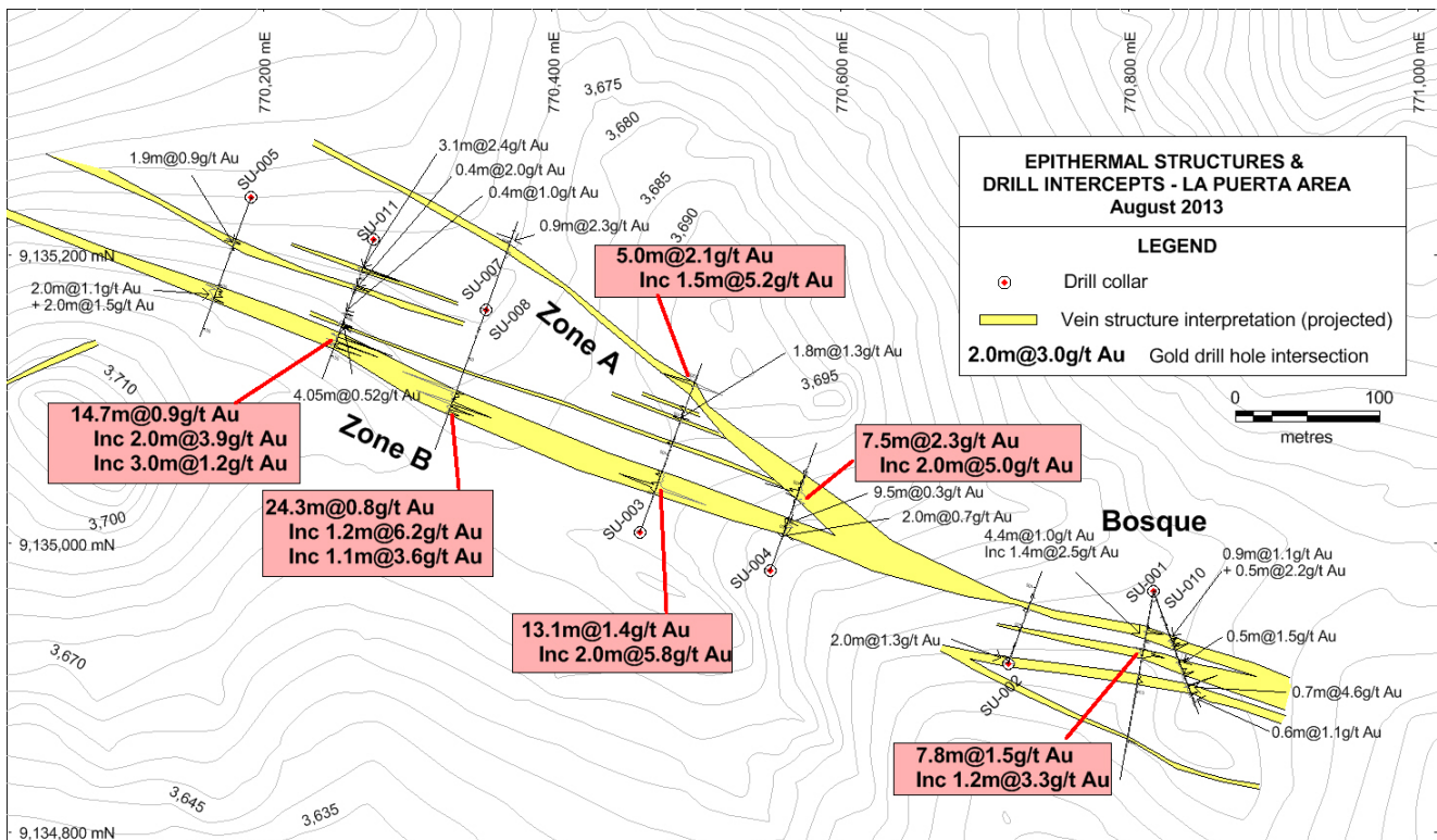
Figure 2. Plan of drill intercepts at La Puerta
