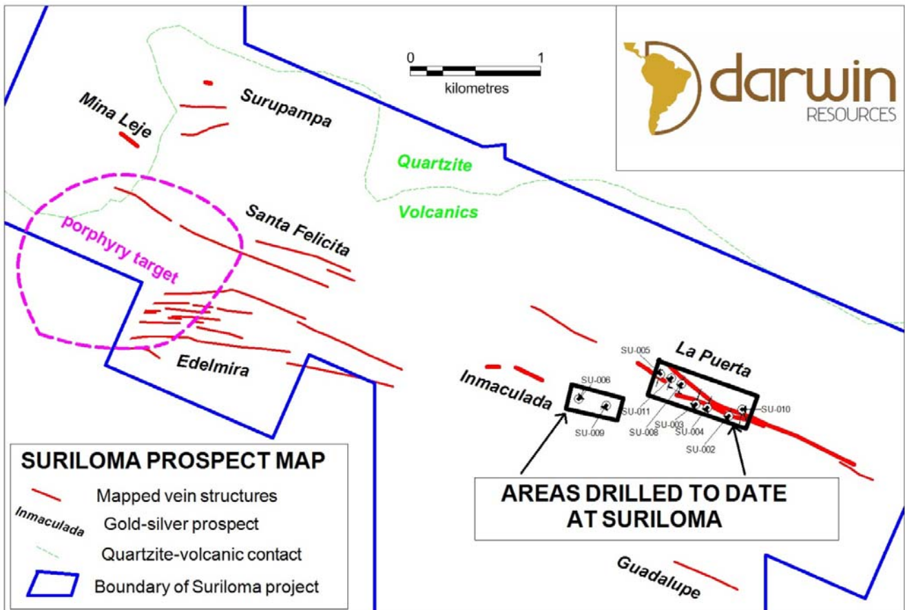
Figure 1. Target areas at Suriloma showing the areas of recent drilling
