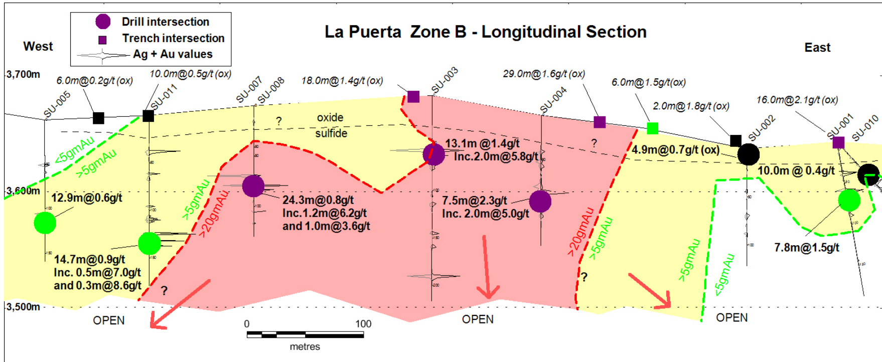
Figure 3. Longitudinal section of La Puerta
