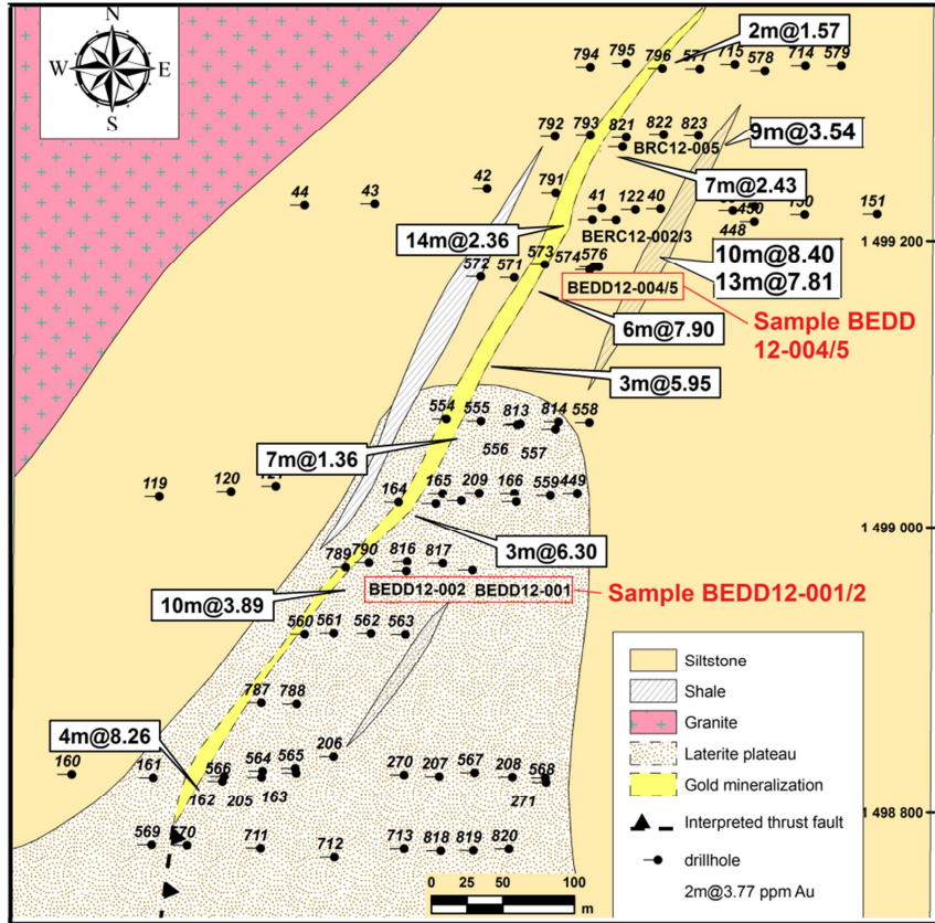
Geological map and drill plan showing the boreholes sampled for metallurgical test work
