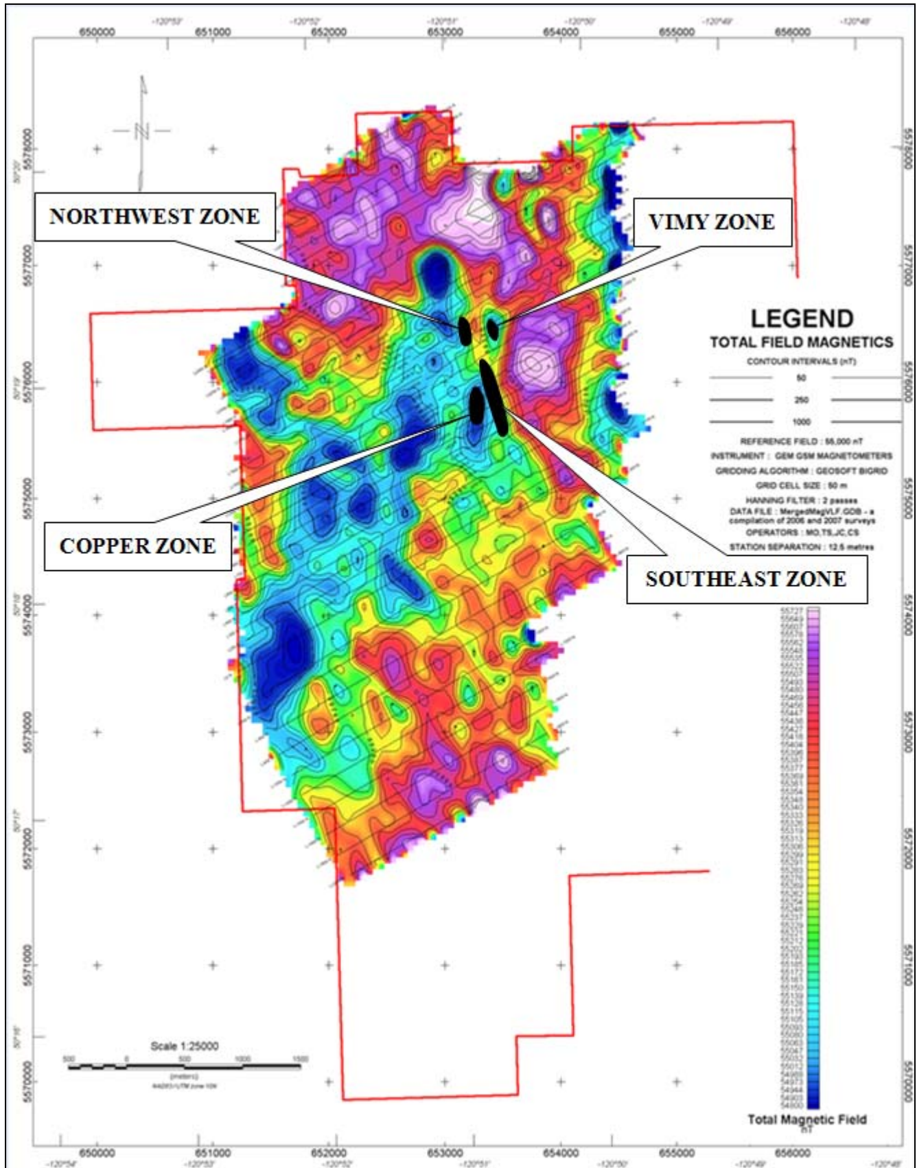
Figure 1 – DOT Property - Total Field Magnetometer Map
