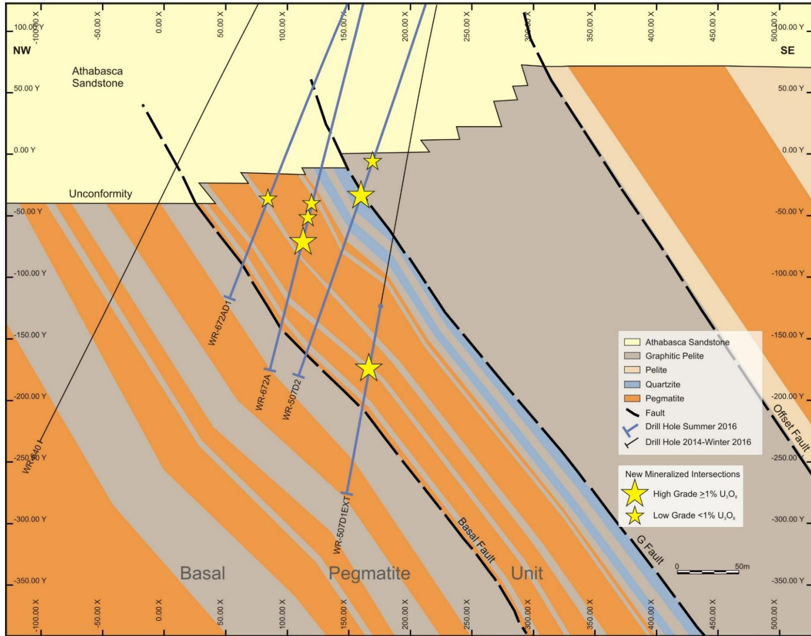
Figure 3: Cross-section along section line 5350 GP, the most northeastern section drilled to date
